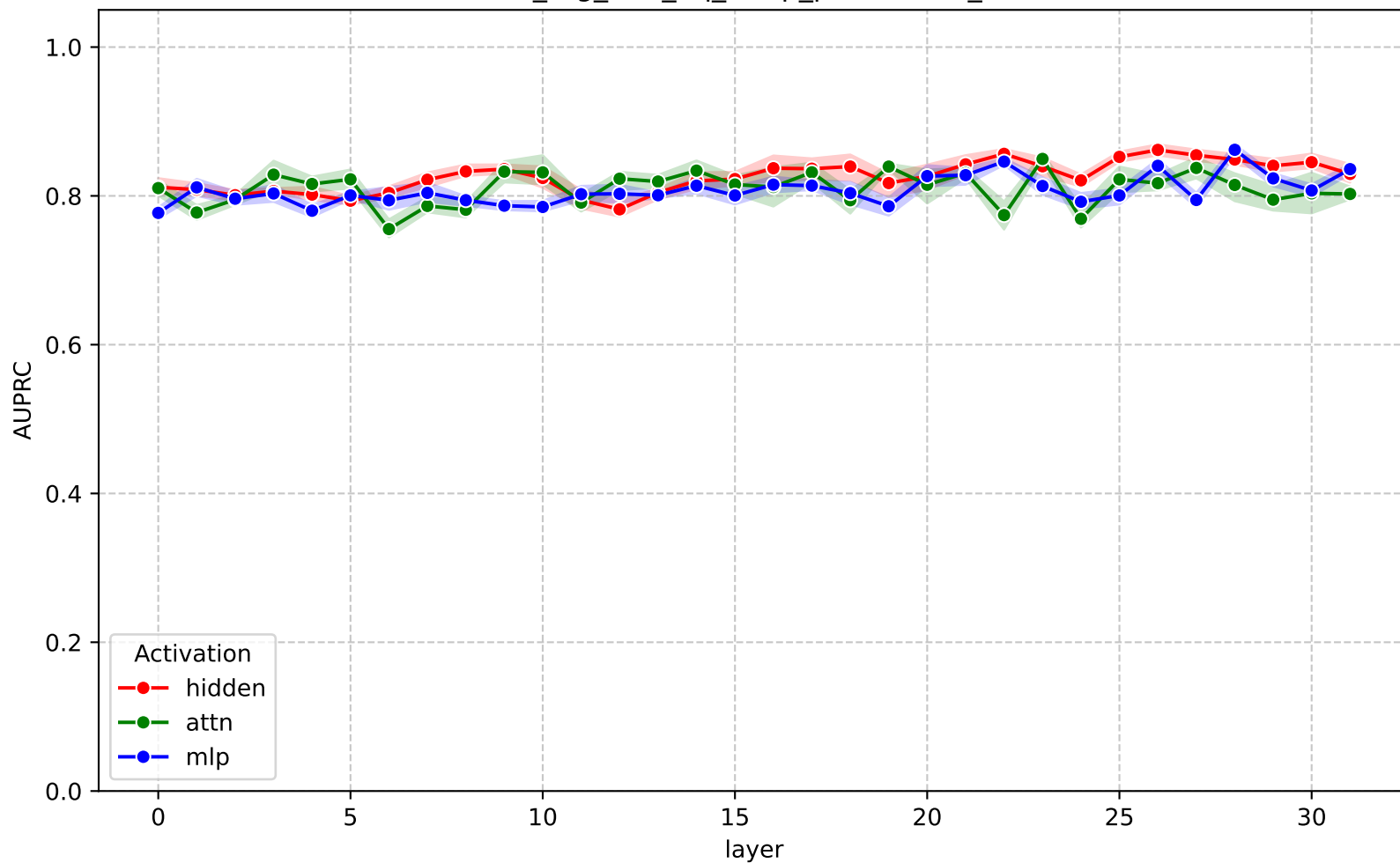
AUPRC across layers - gemma-3-4b-it (train_rag_test_nq_swap_parametric_svm)
