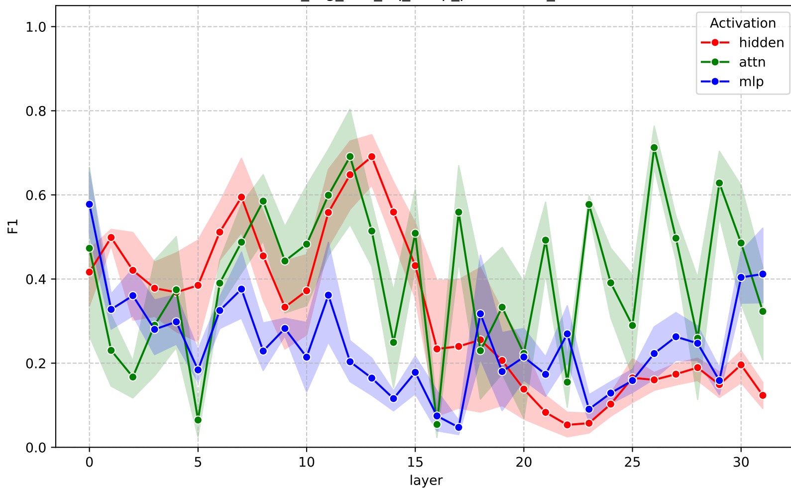
F1 across layers - gemma-3-4b-it (train_rag_test_nq_swap_parametric_svm)
