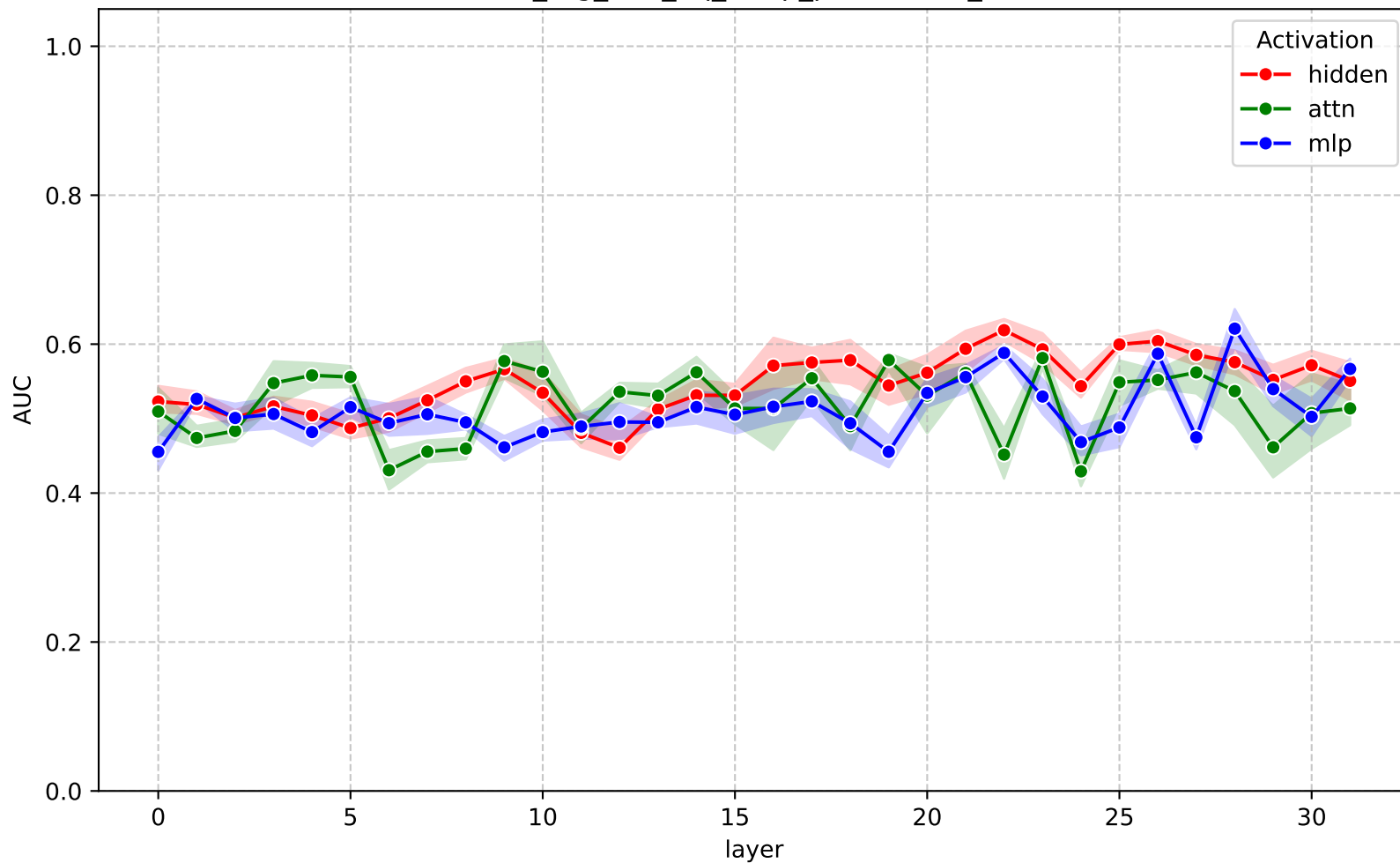
AUC across layers - gemma-3-4b-it (train_rag_test_nq_swap_parametric_svm)
