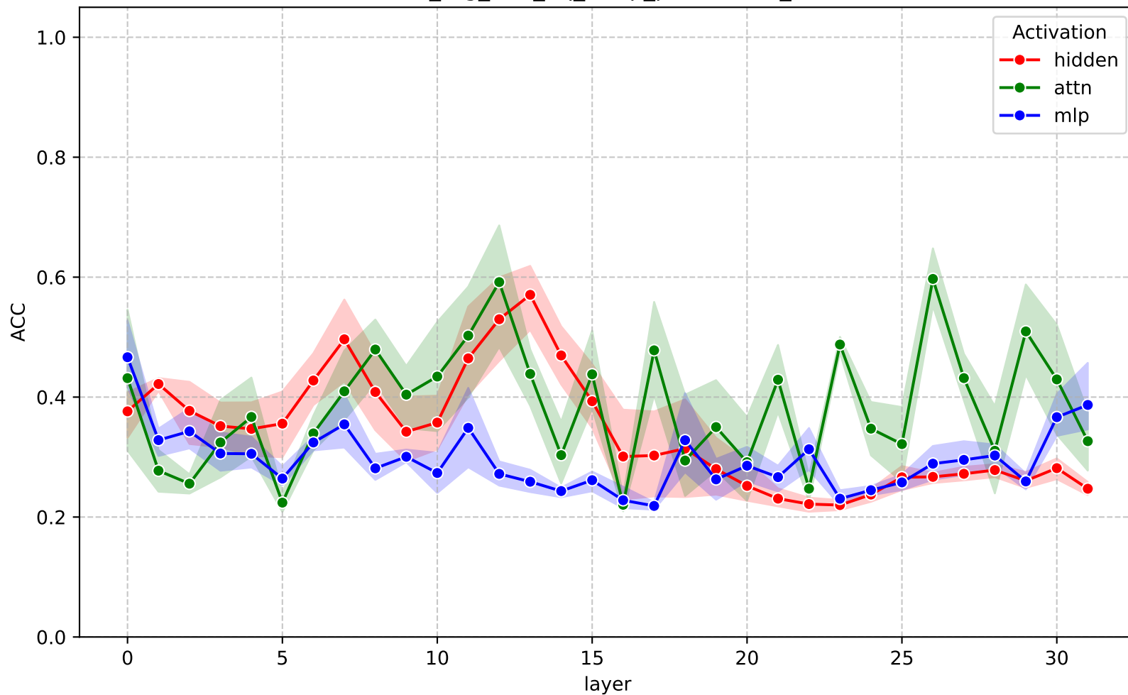
ACC across layers - gemma-3-4b-it (train_rag_test_nq_swap_parametric_svm)
