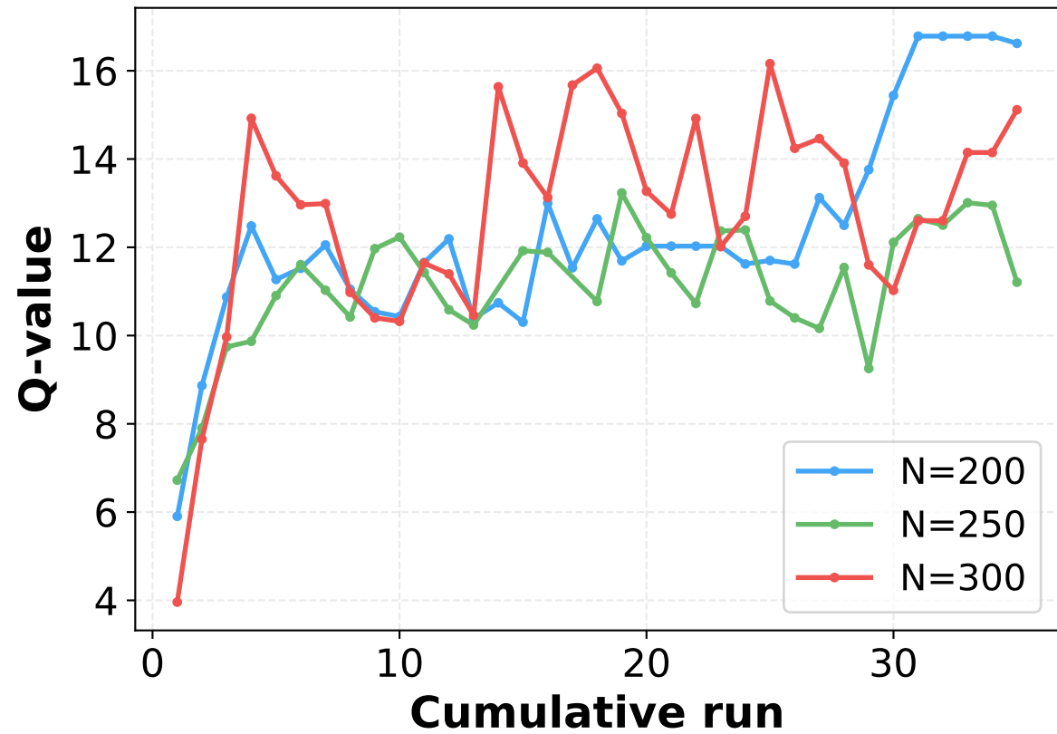
(A) Attacker Q(QUARANTINE)
