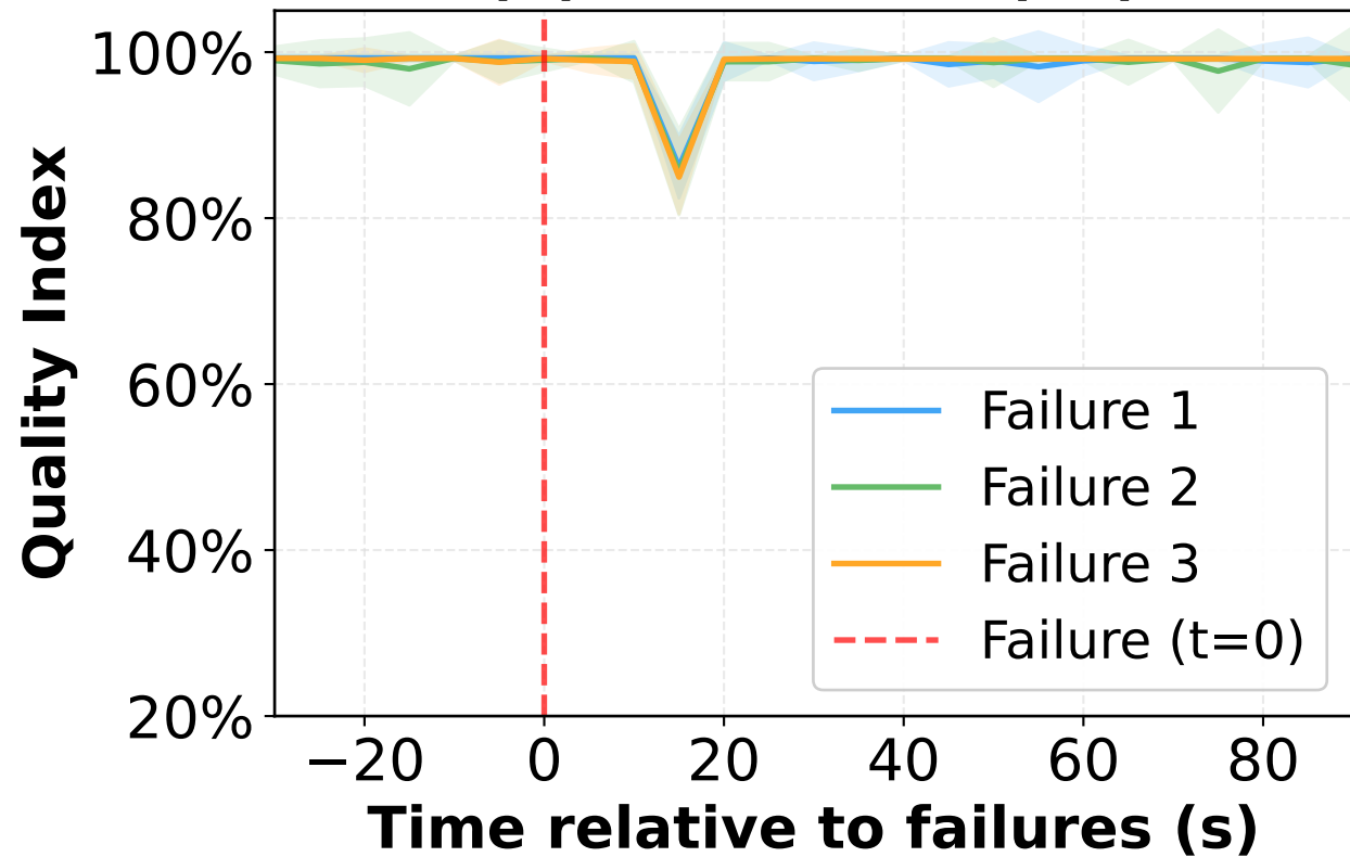
(A) - 250 nodes (FR)
