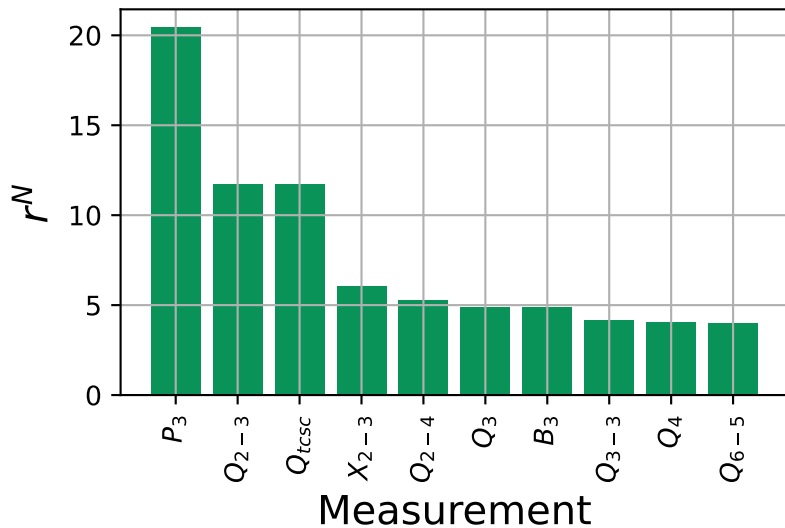
b) FACTS measured
