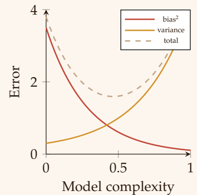
Figure 6: Bias-variance tradeoff: total error has a minimum at optimal capacity.
