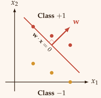
Figure 1: Geometric representation of a linear decision boundary in \mathbb{R}^2 where the weight vector \mathbf{w} acts orthogonal to the separating hyperplane.
