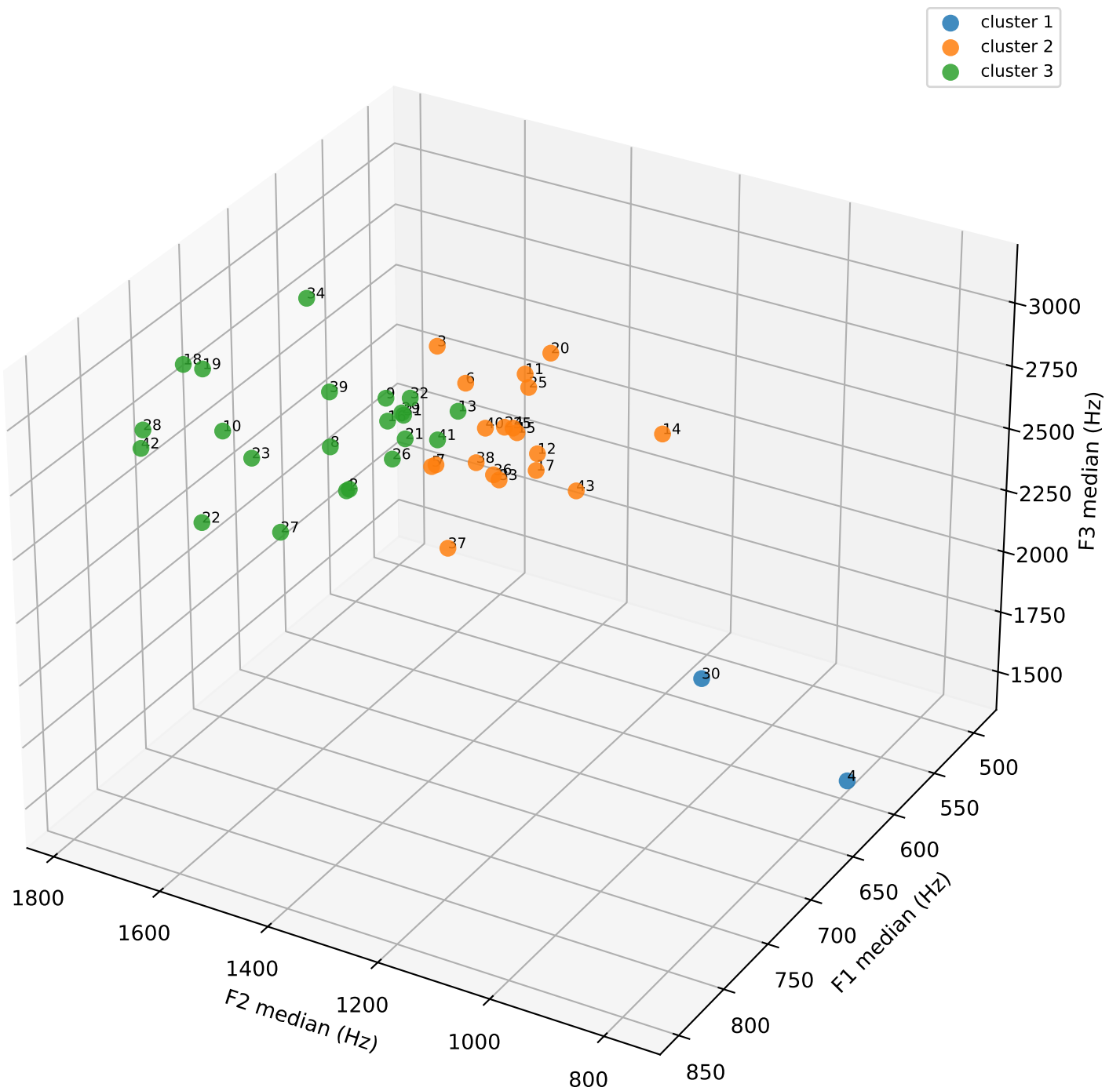
Clusters Ward — voyelle /a/ — F1-F2-F3
