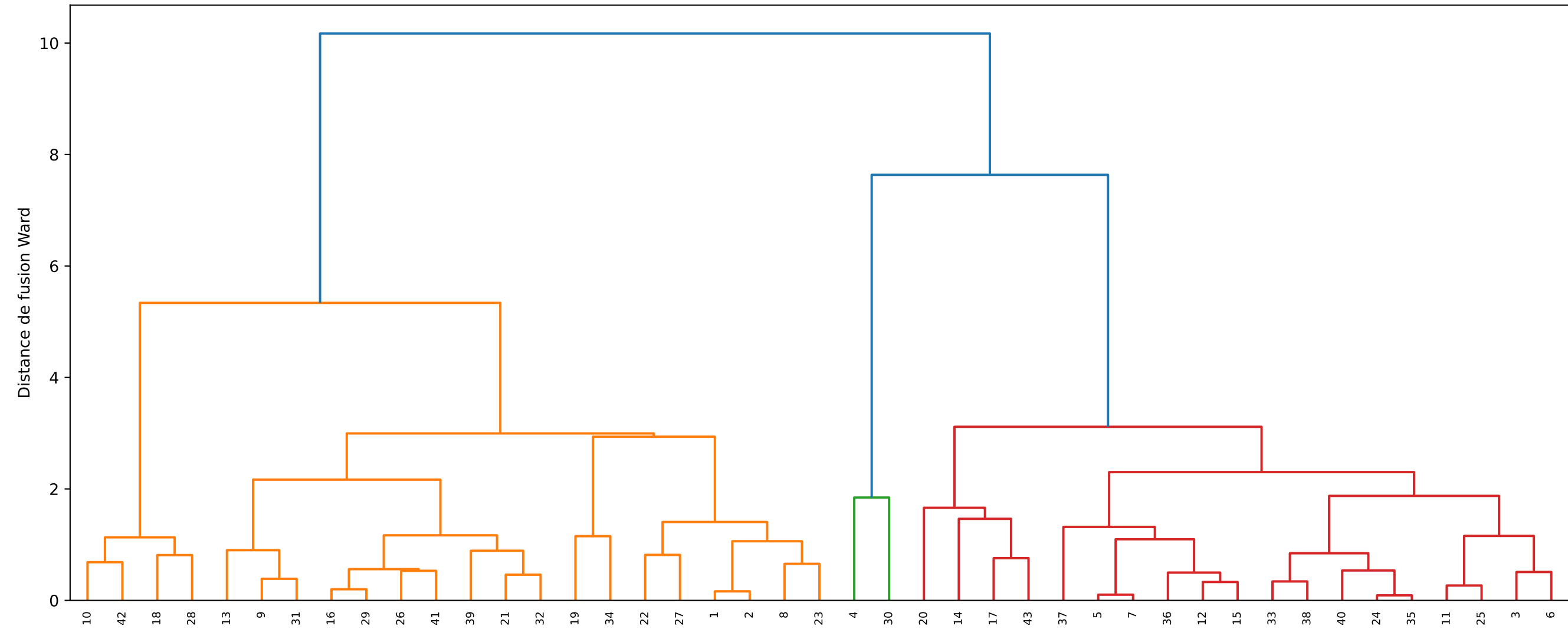
Dendrogramme Ward — voyelle /a/ — F1-F2-F3
