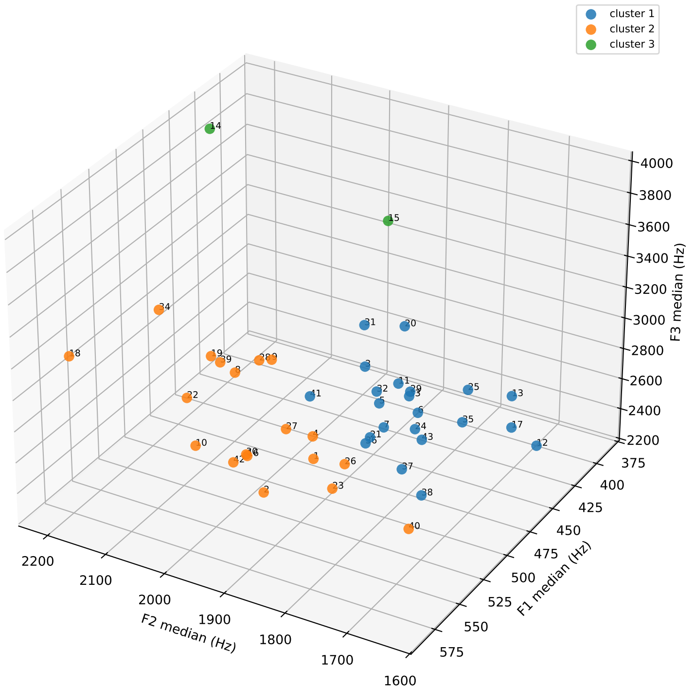
Clusters Ward — voyelle /e/ — F1-F2-F3
