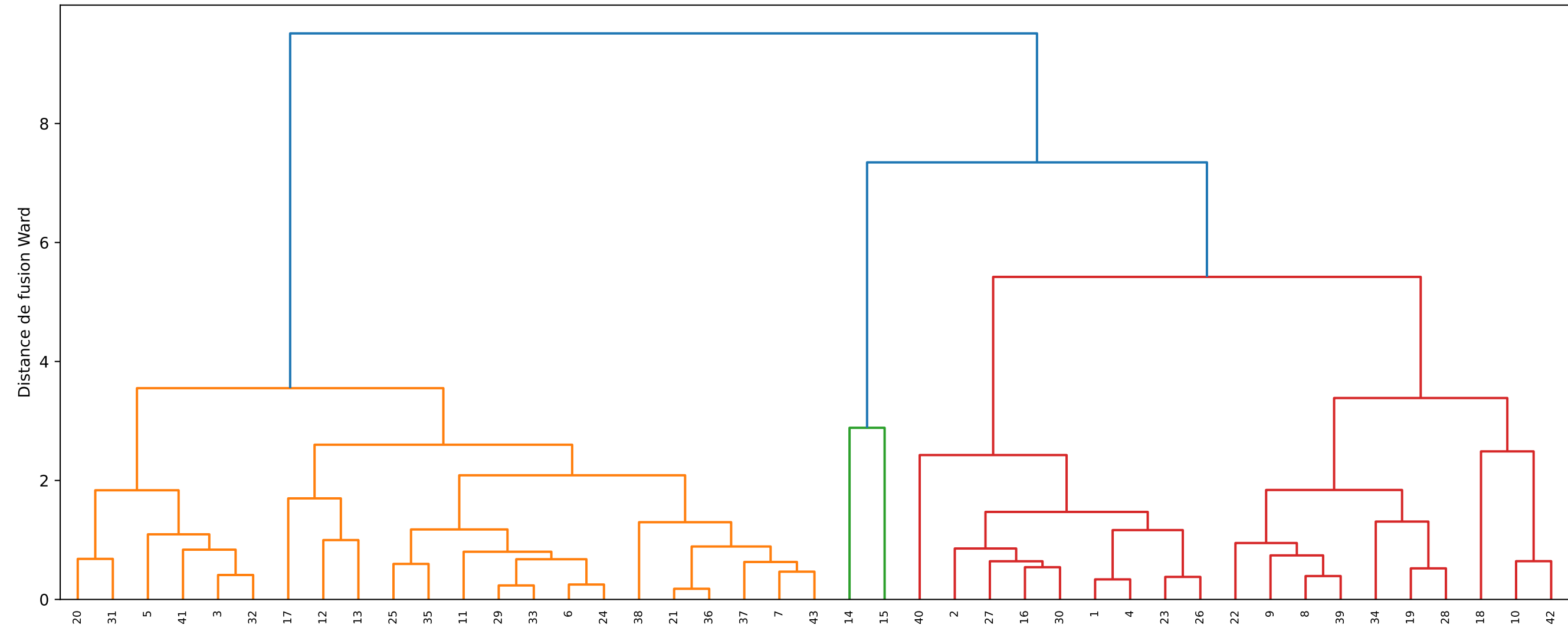
Dendrogramme Ward — voyelle /e/ — F1-F2-F3
