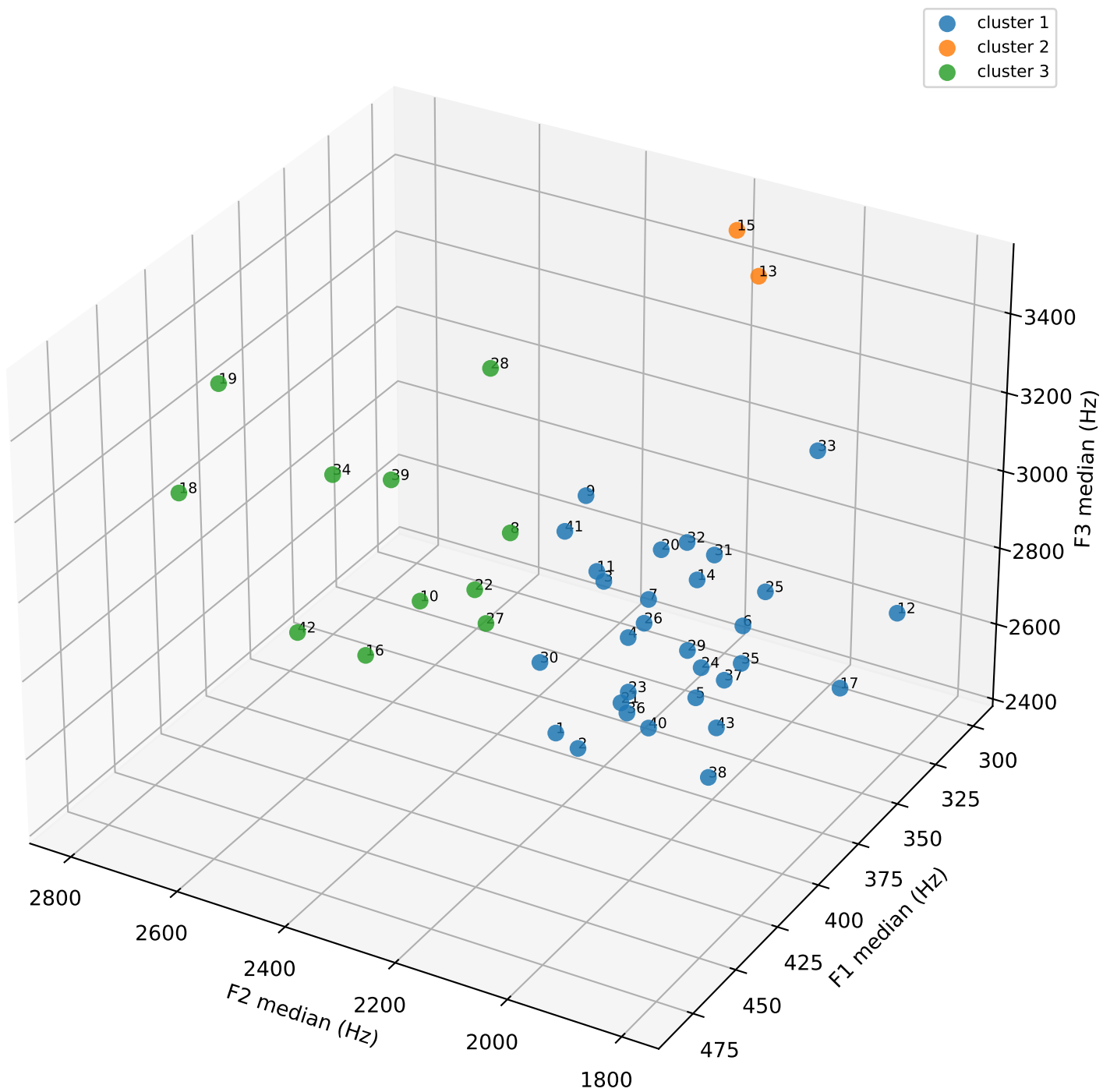
Clusters Ward — voyelle /i/ — F1-F2-F3
