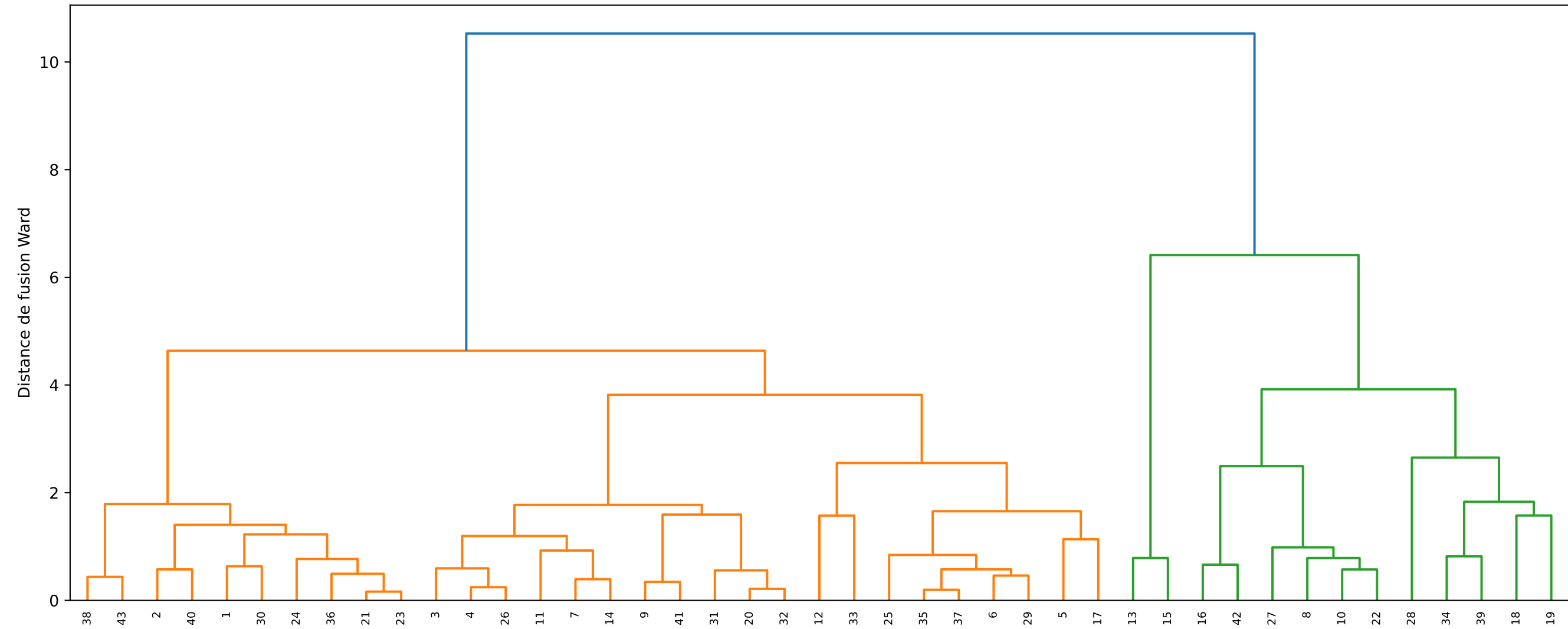
Dendrogramme Ward — voyelle /i/ — F1-F2-F3
