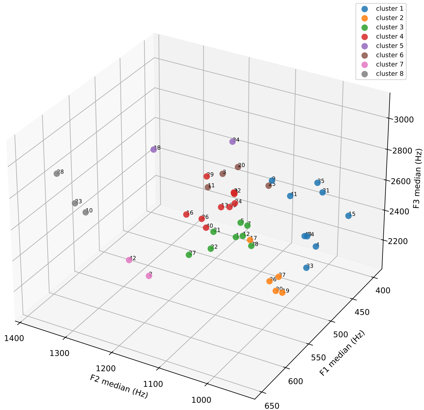
Clusters Ward — voyelle /o/ — F1-F2-F3
