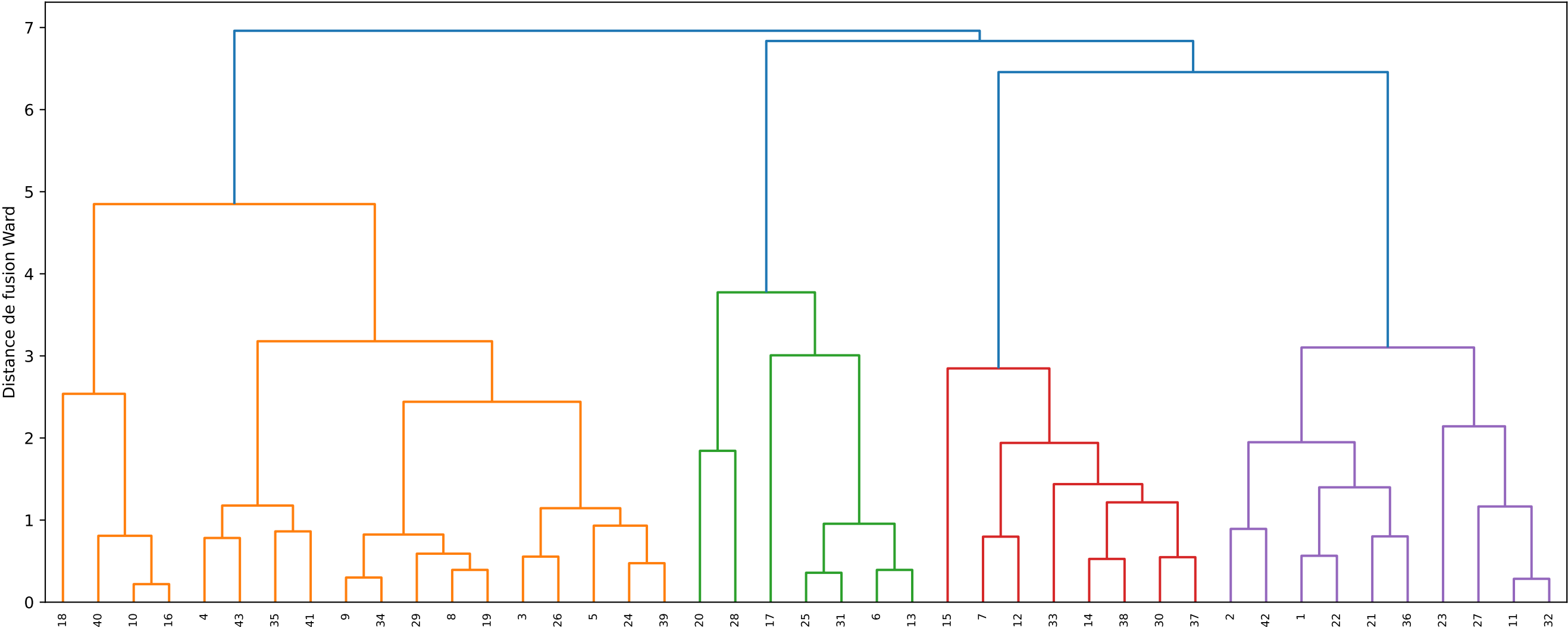
Dendrogramme Ward — voyelle /u/ — F1-F2-F3
