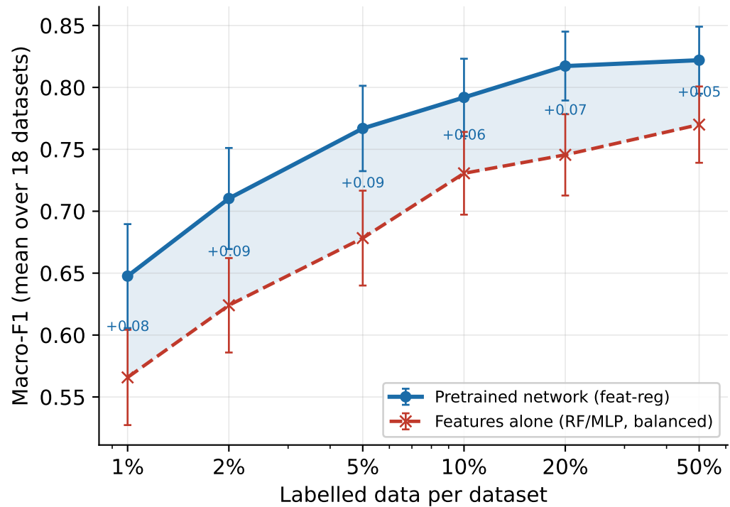
(b) Pretrained network vs. features alone
