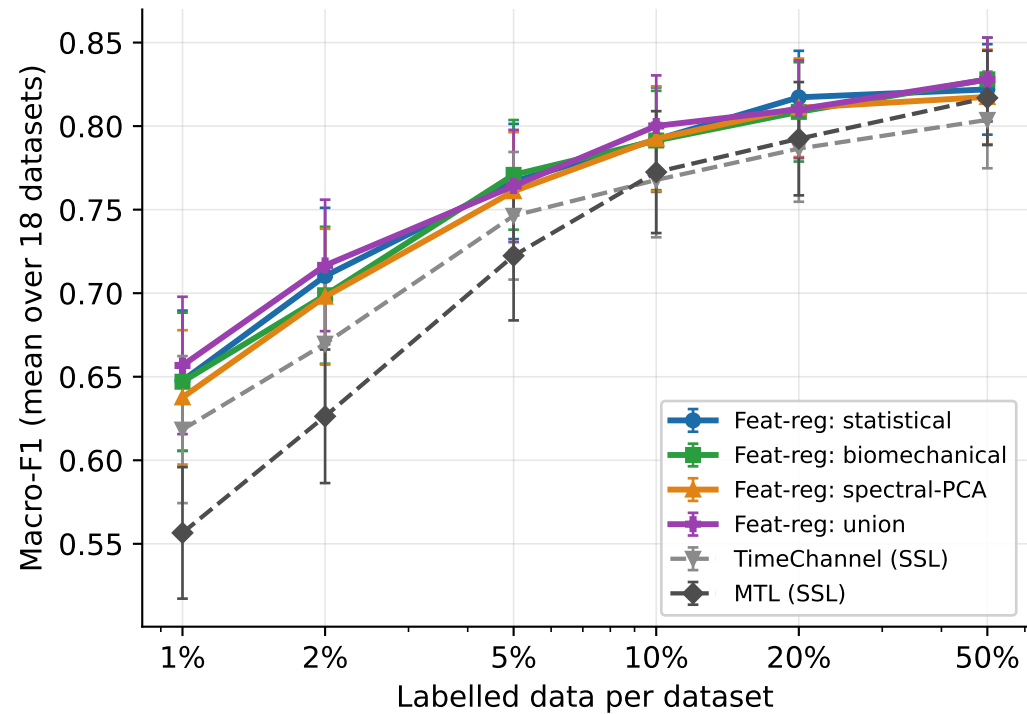
(a) Few-shot: feature-regression vs SSL baselines
