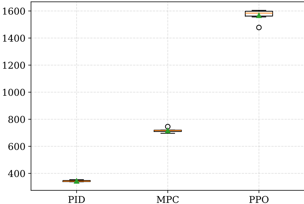
Final Cumulative Energy [J]
