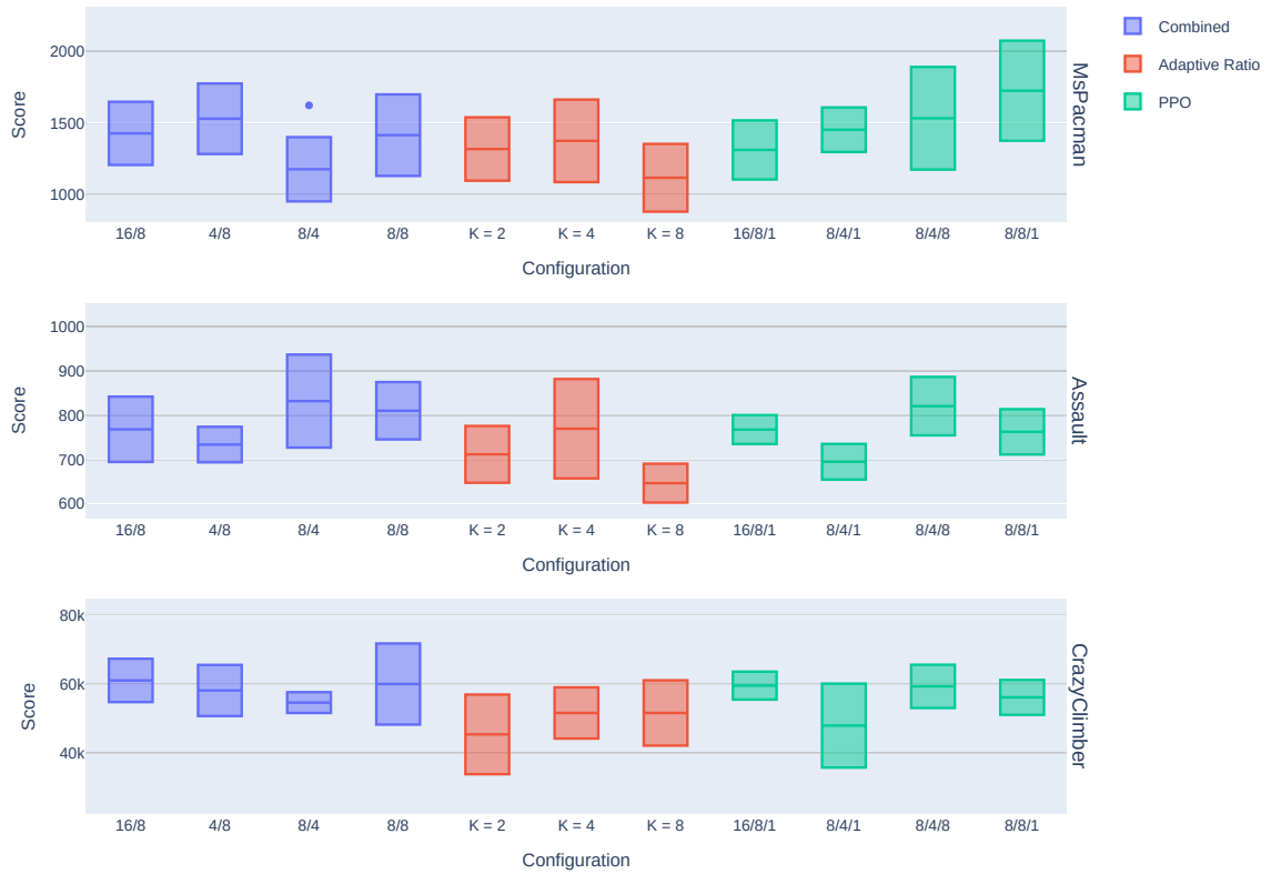
Figure 4.26: A comparison between the results for the adaptive ratio, PPO and their combination. Each row represents a single Atari environment. The boxes, denoting the mean and standard deviation computed across 5 RNG seeds, are placed into three groups, corresponding to the combined test, adaptive model ratio, and PPO. Each box in a given group corresponds to a different hyperparameter preset.
