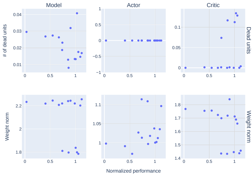
Figure 4.10: Relationship between plasticity-related metrics and agent performance. Rows represent metrics used, while the columns represent the different components (neural networks) measured. The x -axis represents agent performance normalized by the mean score achieved in a non-warm-started setting. The y -axis represents values of the particular metrics.
