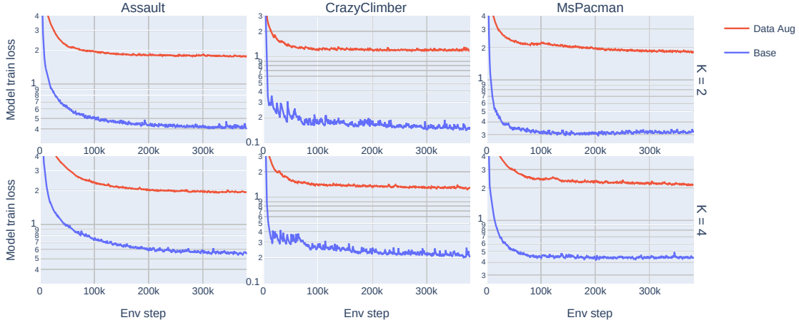
Figure 4.17: A comparison of the model training loss curves for the data-augmented agent, and a non-data-augmented baseline. Each column represents the results for a single environment. Each row corresponds to a different configuration - model/RL update ratio used. In each subplot, curves for the data-augmented and non-data-augmented variants are displayed. The curves have been smoothed by exponential moving average, to improve the clarity of the presentation.
