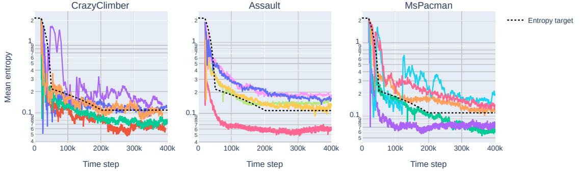
Figure 4.23: Mean policy entropy curves for the best-performing agents in the baseline experiment. Each Atari environment is represented by a different subplot. The x -axis denotes the number of environment step passed. The y -axis represents the mean policy entropy. Each solid line represents a different training run. The dashed line denotes an example entropy schedule approximating these schedules.
