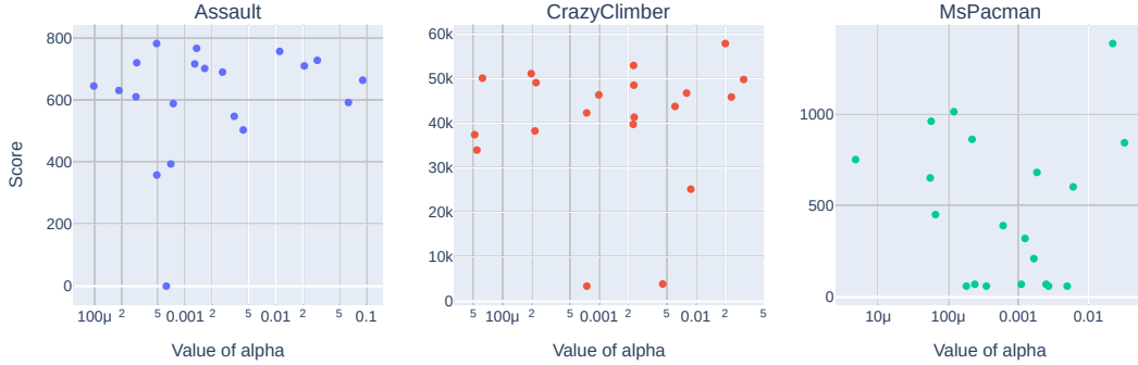
Figure 4.21: Relationship between SAC’s \alpha value, and the agent performance. Each subplot contains the results for a different Atari environment. Each point represents a single training run. The x -axis denotes the value of \alpha parameter used in the test. The y -axis signifies the final validation score obtained by the agent.
