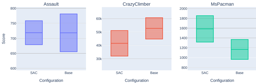
Figure 4.24: A comparison between the baseline experiment and the experiment with SAC and a user-defined entropy schedule. Each Atari environment tested is represented by a single subplot. The boxes denote the mean and the standard deviation of the final validation score, estimated with 5 training runs per configuration.
