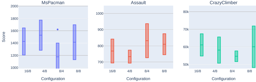
Figure 4.25: A comparison between the different hyperparameter presets for the experiment combining improvements in the context of a single agent.
