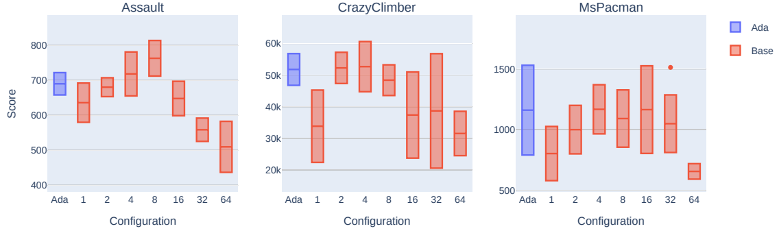
Figure 4.11: The comparison of the final validation scores, for the adaptive ratio experiment Ada and the baseline experiments 1 - 64, where the number denotes the model/RL update ratio K . Each subplot shows the results for a different environment tested. The bars signify mean and one standard deviation, obtained from a sample of 5 training runs for each configuration.
