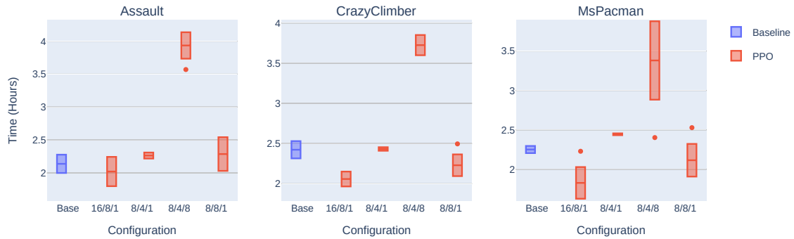
Figure 4.20: Comparison of the total training run durations for the baseline and a number of different configurations of PPO. Each subplot contains the results for a different Atari environment. Each box represents the mean and the standard deviation computed across 5 training runs.
