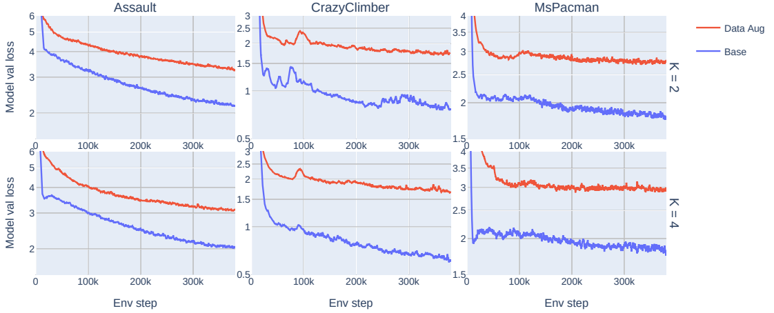
Figure 4.16: A comparison of the model validation loss curves for the data-augmented agent, and a non-data-augmented baseline. Each column represents the results for a single environment. Each row corresponds to a different configuration - model/RL update ratio used. In each subplot, curves for the data-augmented and non-data-augmented variants are displayed. The curves have been smoothed by exponential moving average, to improve the clarity of the presentation.
