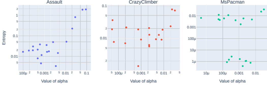
Figure 4.22: Relationship between SAC’s \alpha value, and the final mean policy entropy. Each subplot contains the results for a different Atari environment. Each point represents a single training run. The x -axis denotes the value of \alpha parameter used in the test. The y -axis signifies the final value of the mean policy entropy metric.
