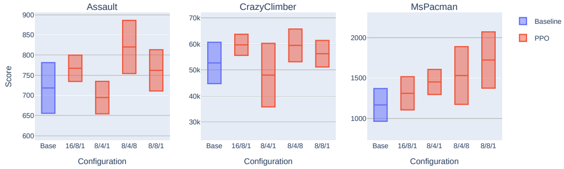
Figure 4.19: Comparison of the final validation scores between the baseline and a number of different configurations of PPO. Each subplot contains the results for a different Atari environment. Each box represents the mean and the standard deviation computed across 5 training runs.
