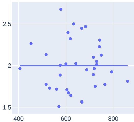
Assault
