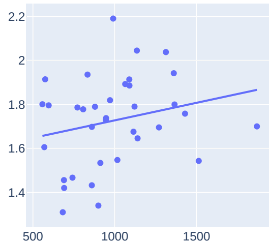
MsPacman
