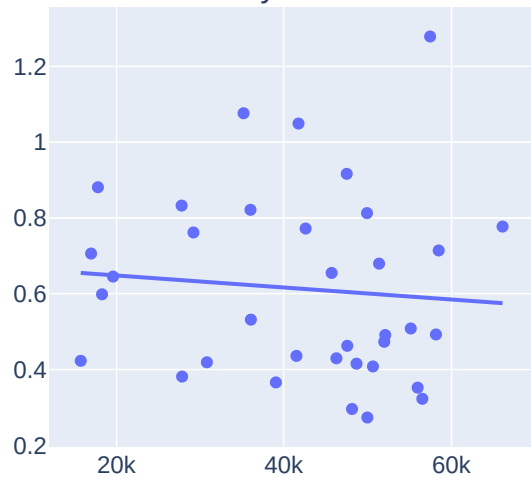
CrazyClimber
