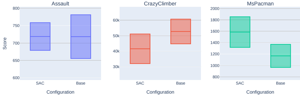
Figure 4.20: A comparison between the baseline experiment and the experiment with SAC and a user-defined entropy schedule. Each Atari environment tested is represented by a single subplot. The boxes denote the mean and the standard deviation of the final validation score, estimated with 5 training runs per configuration.
