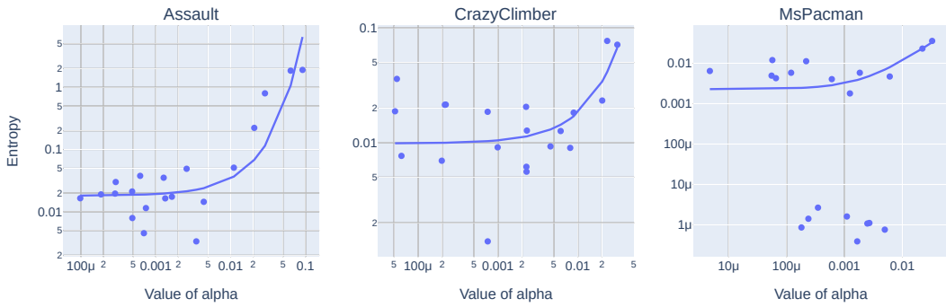
Figure 4.20: Relationship between SAC's \alpha value, and the final mean policy entropy. Each subplot contains the results for a different Atari environment. Each point represents a single training run. The x -axis denotes the value of \alpha parameter used in the test. The y -axis signifies the final value of the mean policy entropy metric.
