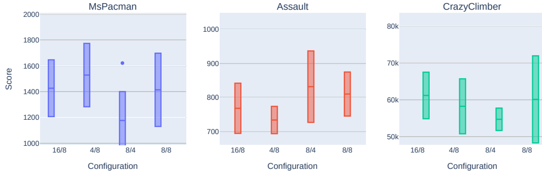
Figure 4.23: A comparison between the different hyperparameter presets for the experiment combining improvements in the context of a single agent.
