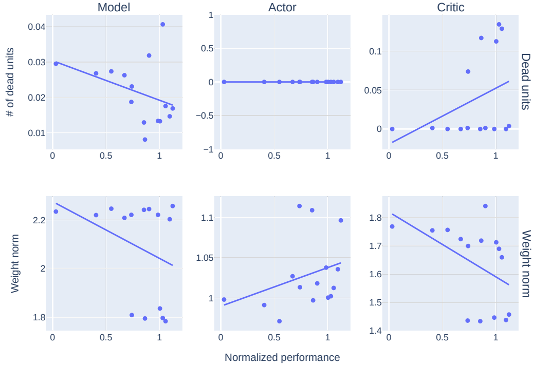
Figure 4.8: Relationship between plasticity-related metrics and agent performance. Rows represent metrics used, while the columns represent the different components (neural networks) measured. The x -axis represents agent performance normalized by the mean score achieved in a non-warm-started setting. The y -axis represents values of the particular metrics.
