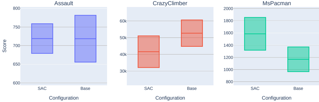
Figure 4.22: A comparison between the baseline experiment and the experiment with SAC and a user-defined entropy schedule. Each Atari environment tested is represented by a single subplot. The boxes denote the mean and the standard deviation of the final validation score, estimated with 5 training runs per configuration.
