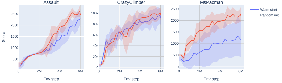
Figure 4.7: A comparison of the validation scores for the warm-started agents, and the ones with parameters initialized randomly. The lines show the mean and the standard deviation of agent validation scores, measured across 5 RNG seeds.
