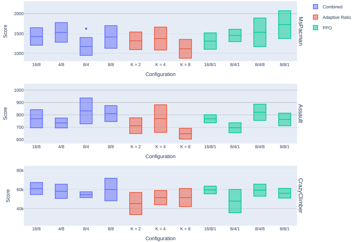
Figure 4.24: A comparison between the results for the adaptive ratio, PPO and their combination. Each row represents a single Atari environment. The boxes, denoting the mean and standard deviation computed across 5 RNG seeds, are placed into three groups, corresponding to the combined test, adaptive model ratio, and PPO. Each box in a given group corresponds to a different hyperparameter preset.
