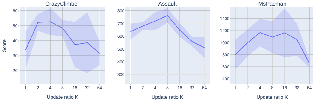
Figure 4.3: Final test episode returns for each of the 3 tested environments, relative to the data-to-update ratio K . The line indicates the mean across the RNG seeds, and the shaded area indicates the standard deviation. Note: The x-axis is logarithmic.
