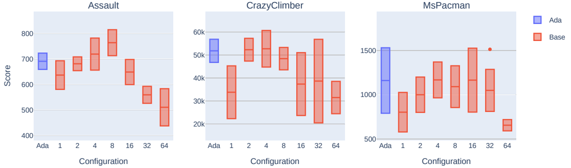
Figure 9: The comparison of the final validation scores, for the adaptive ratio experiment Ada and the baseline experiments 1 - 64, where the number denotes the model/RL update ratio K . Each subplot shows the results for a different environment tested. The bars signify mean and one standard deviation, obtained from a sample of 5 training runs for each configuration.
