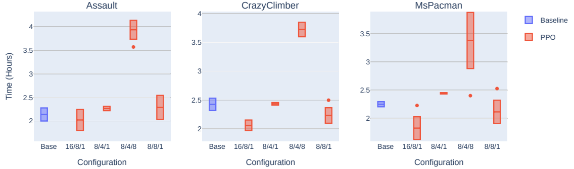
Figure 18: Comparison of the total training run durations for the baseline and a number of different configurations of PPO. Each subplot contains the results for a different Atari environment. Each box represents the mean and the standard deviation computed across 5 training runs.
