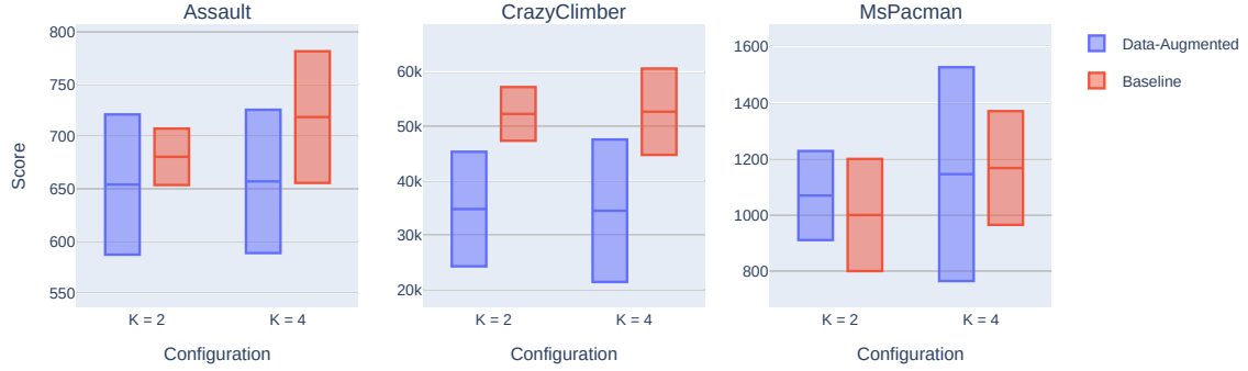
Figure 13: A comparison of the final validation scores for the data-augmented agent, and a non-data-augmented baseline. Each subplot represents the results for a single environment. In each subplot, results for different values of model/RL update ratio K are grouped together. Each group contains a box, signifying the mean and the standard deviation evaluated across 5 training runs, for the data-augmented and the non-data-augmented variants.
