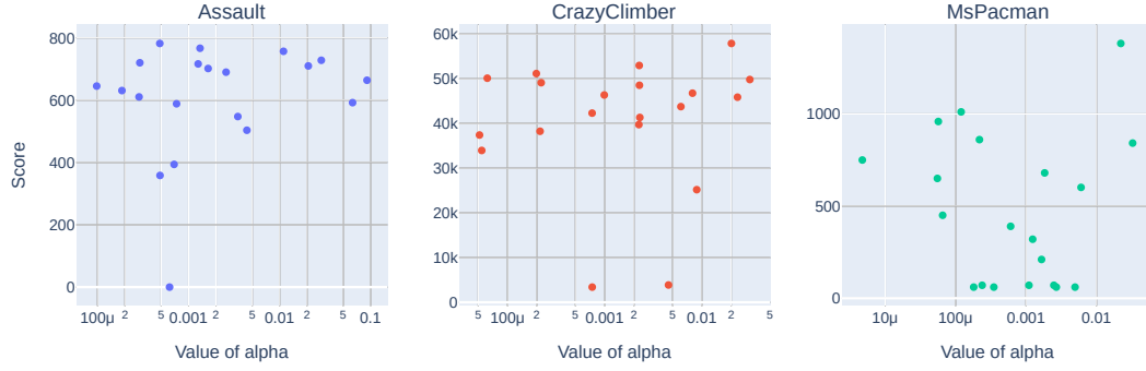
Figure 19: Relationship between SAC’s \alpha value, and the agent performance. Each subplot contains the results for a different Atari environment. Each point represents a single training run. The x -axis denotes the value of \alpha parameter used in the test. The y -axis signifies the final validation score obtained by the agent.
