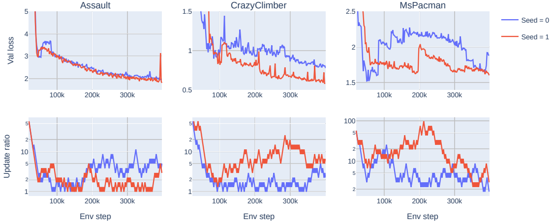
Figure 11: The curves for the model validation loss and the current update ratio, for the adaptive ratio experiment. Each column represents a different Atari task. Two training runs, corresponding to two different RNG seeds, are shown on each subplot. The model validation curves have been smoothed with exponential moving average to improve the clarity of the presentation.
