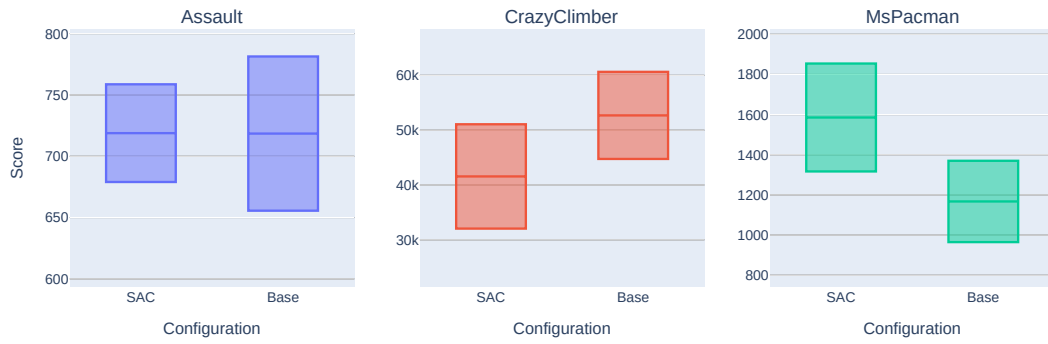
Figure 22: A comparison between the baseline experiment and the experiment with SAC and a user-defined entropy schedule. Each Atari environment tested is represented by a single subplot. The boxes denote the mean and the standard deviation of the final validation score, estimated with 5 training runs per configuration.
