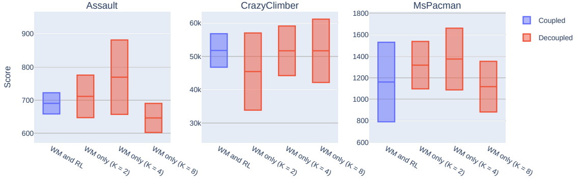
Figure 12: A comparison between the final validation scores for the coupled and the decoupled variants of the adaptive update ratio experiment. Each subplot represents a different environment tested. Each box signifies the results for a given configuration - mean and one standard deviation, obtained from a sample of 5 training runs for each configuration.
