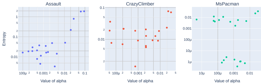
Figure 20: Relationship between SAC’s \alpha value, and the final mean policy entropy. Each subplot contains the results for a different Atari environment. Each point represents a single training run. The x -axis denotes the value of \alpha parameter used in the test. The y -axis signifies the final value of the mean policy entropy metric.
