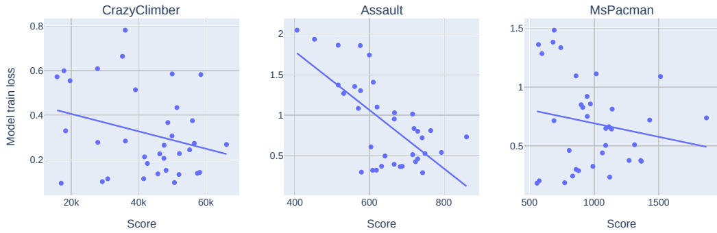
Figure 7: Relationship between final validation score and final model training loss. Each point represents a single training run. The x-axis represents the agent performance. The y-axis represents the value of the model training loss at the end of the training.
