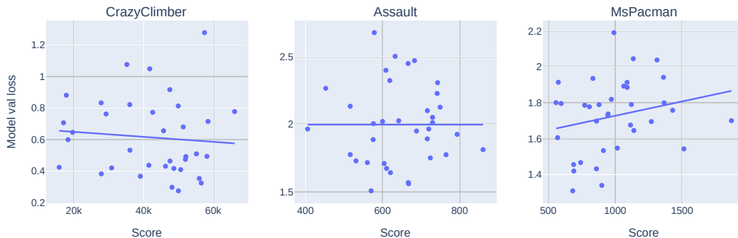
Figure 5: Relationship between final validation score and final model validation loss. Each point represents a single training run. The x-axis represents the agent performance. The y-axis represents the value of the model validation loss at the end of the training.
