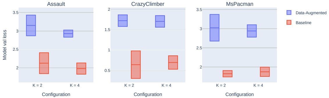
Figure 14: A comparison of the final model validation loss values for the data-augmented agent, and a non-data-augmented baseline. Each subplot represents the results for a single environment. In each subplot, results for different values of model/RL update ratio K are grouped together. Each group contains a box, signifying the mean and the standard deviation evaluated across 5 training runs, for the data-augmented and the non-data-augmented variants.
