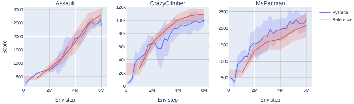
Figure 2: Comparison of the validation scores for Tensorflow and Pytorch versions. Note: The scores for the reference (Tensorflow) version have been supplied by the authors, and were not verified independently.
