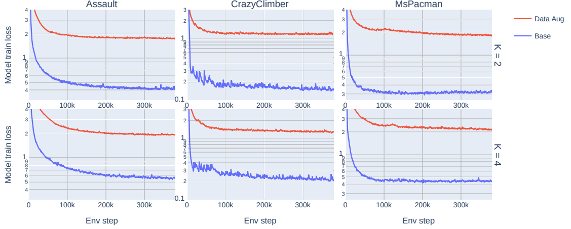
Figure 15: A comparison of the model training loss curves for the data-augmented agent, and a non-data-augmented baseline. Each column represents the results for a single environment. Each row corresponds to a different configuration - model/RL update ratio used. In each subplot, curves for the data-augmented and non-data-augmented variants are displayed. The curves have been smoothed by exponential moving average, to improve the clarity of the presentation.
