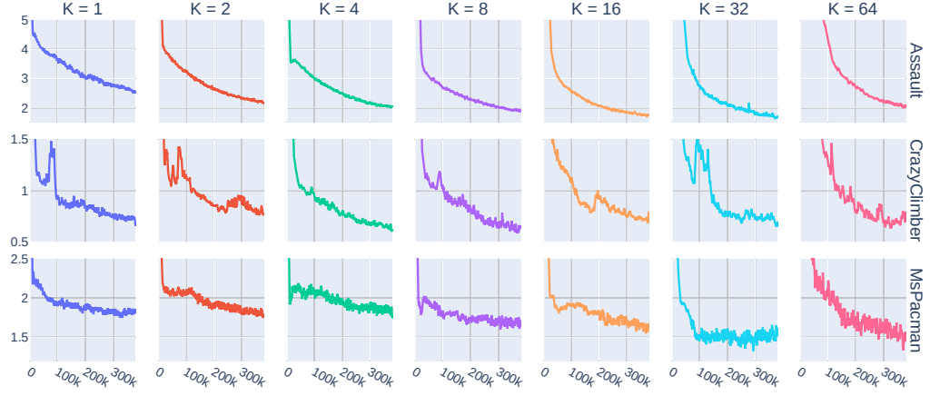
Figure 6: Averaged model validation loss curves for each configuration of the environment and the update ratio used. Rows represent different environments, and the columns the different update ratios used. The x-axis corresponds to the number of environment steps taken, and the y-axes represent loss values. The ranges of the y-axes are different for each environment.
