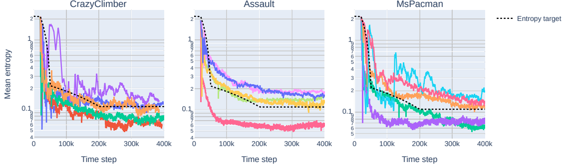
Figure 21: Mean policy entropy curves for the best-performing agents in the baseline experiment. Each Atari environment is represented by a different subplot. The x -axis denotes the number of environment step passed. The y -axis represents the mean policy entropy. Each solid line represents a different training run. The dashed line denotes an example entropy schedule approximating these schedules.
