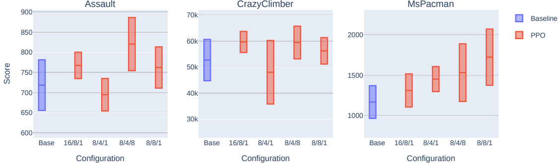
Figure 17: Comparison of the final validation scores between the baseline and a number of different configurations of PPO. Each subplot contains the results for a different Atari environment. Each box represents the mean and the standard deviation computed across 5 training runs.
