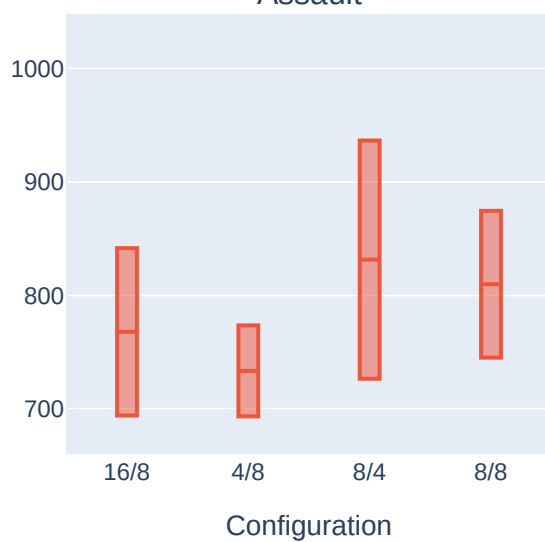
Assault
