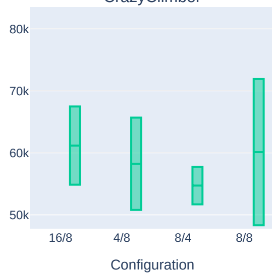
CrazyClimber
