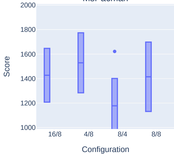
MsPacman
