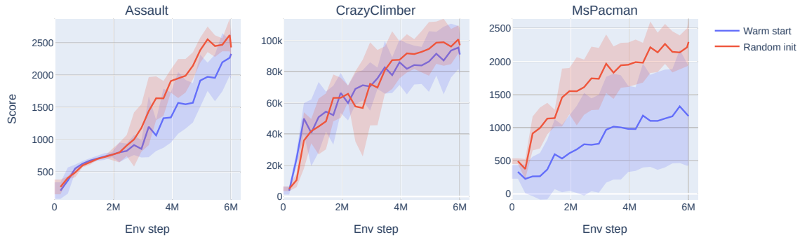
Figure 4.9: A comparison of the validation scores for the warm-started agents, and the ones with parameters initialized randomly. The lines show the mean and the standard deviation of agent validation scores, measured across 5 RNG seeds.
