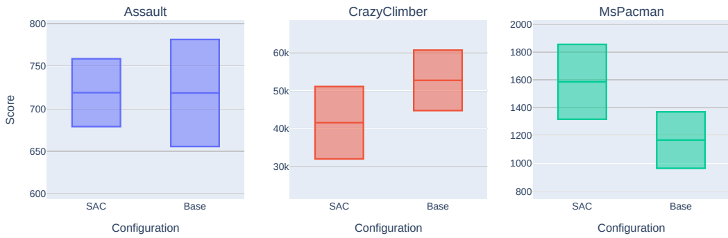
Figure 4.23: A comparison between the baseline experiment and the experiment with SAC and a user-defined entropy schedule. Each Atari environment tested is represented by a single subplot. The boxes denote the mean and the standard deviation of the final validation score, estimated with 5 training runs per configuration.
