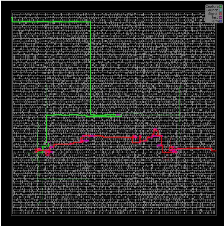
Figure 1: ORFS GUI export final_worst_path of the sep layout (TT, 7.2 ns): the worst setup path runs from the east-edge port in_a[27] to the copy-A fence at the west edge. Source final_worst_path.webp.png (= build/pd_sep/reports/sky130hd/orbit_demo/sep/final_worst_path.webp.png ).
