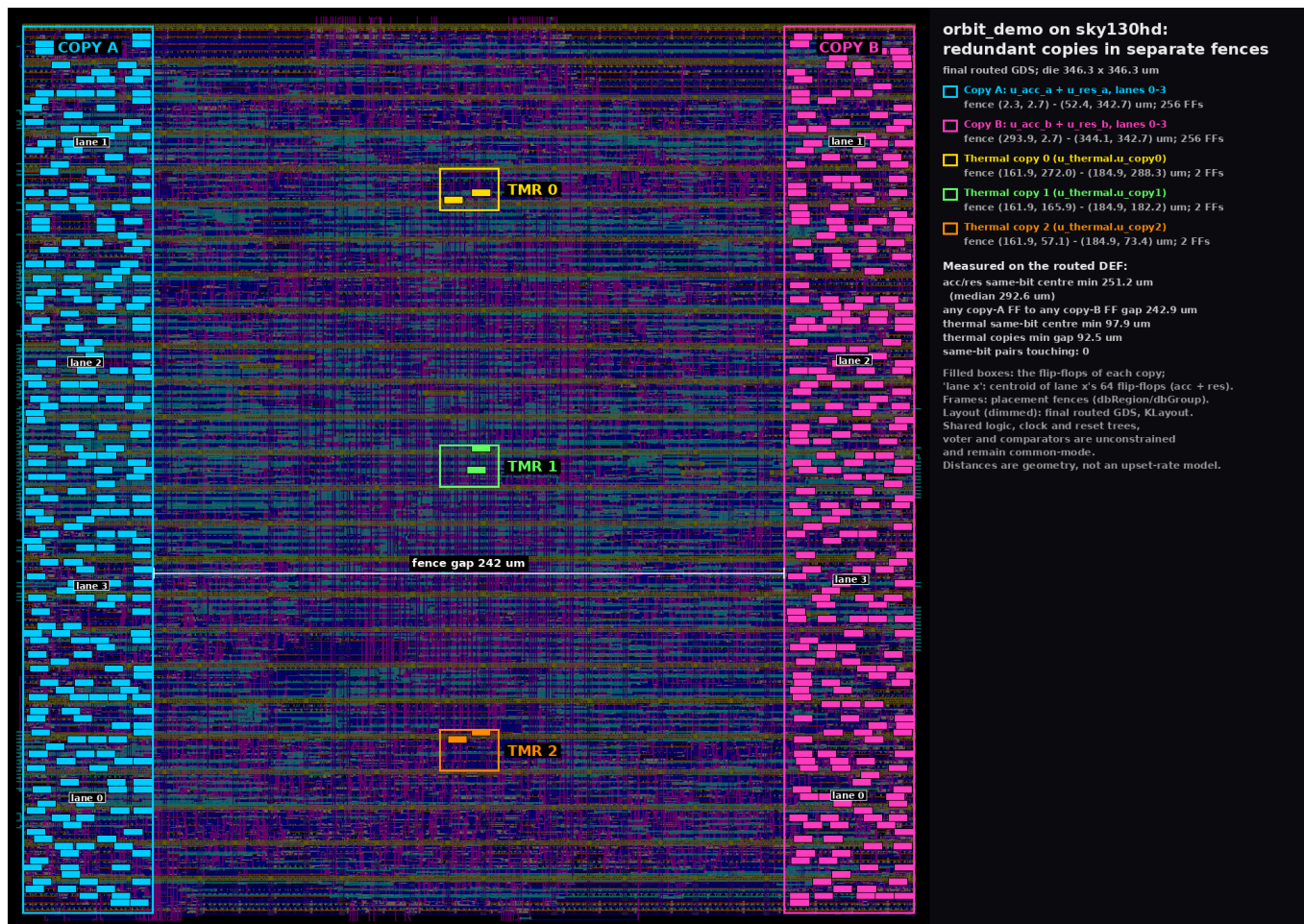
Figure 1. Routed sep GDS (KLayout render by scripts/pdsep_render.py , published as orbit_demo_sky130hd_sep.png ). Copy A and copy B fences at the die edges, thermal fences TMR 0-2 in the centre column. Everything between the fences (multipliers, adders, comparators, OR-tree, voter, clock and reset trees) is shared (K-02). The "fence gap 242 um" label rounds the measured 241.50 um (D-13). Status: VERIFIED.
