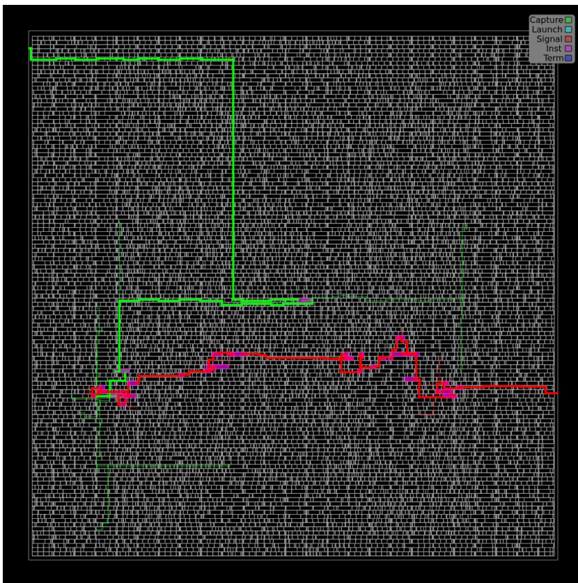
final_worst_path.webp.png: worst setup path (gui::show_worst_path): data path (red) from in_a[27] on the E edge to g_lane[3].u_lane.u_res_a/q[29] in the copy-A fence; launch/capture clock paths in green; slack 0.03 ns at 7.2 ns, TT ( worst_setup_path.txt ).
