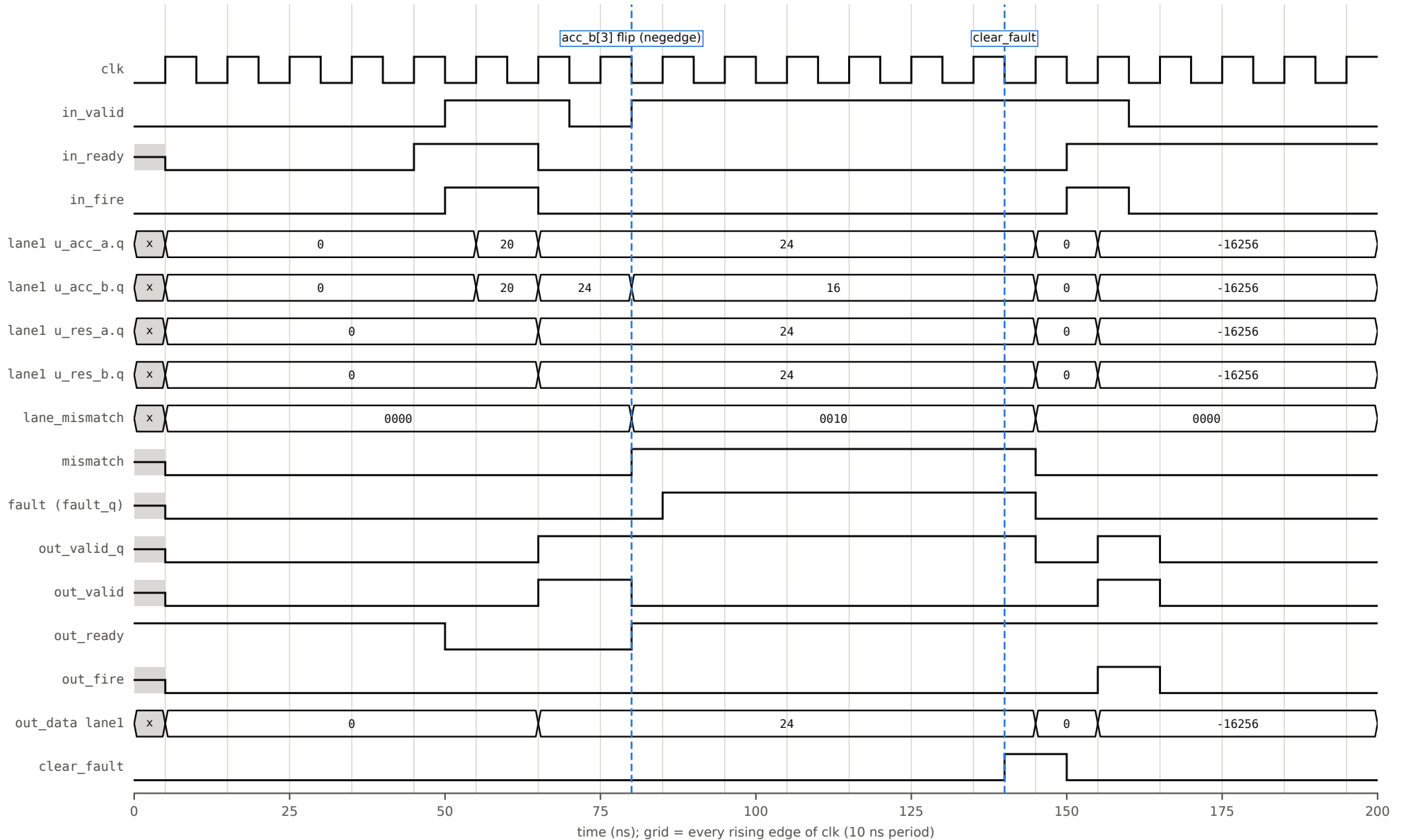
(c) single-bit upset in g_lane[1].u_lane.u_acc_b.q, fault-stop, clear_fault recovery
