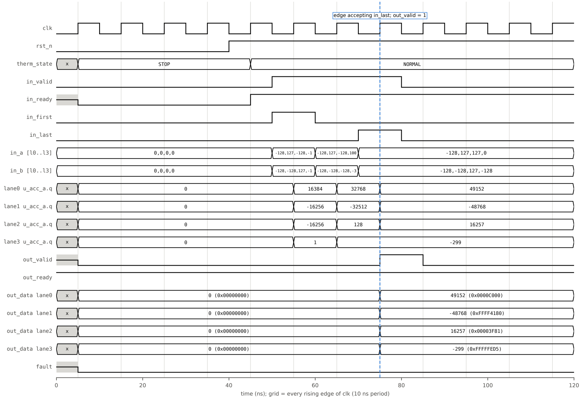
(a) reset, then a 3-beat MAC on all 4 lanes (in_first .. in_last), signed edge cases
