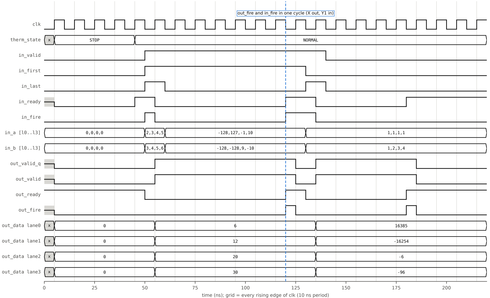
(b) output backpressure: out_ready low with a full buffer, then drain and refill
