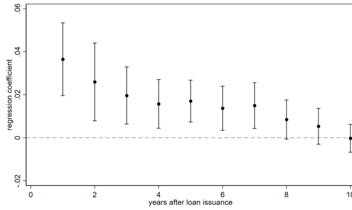
Figure 3: Correlation between rate residuals and unexpected changes in default probability, by year. Balanced sample.
