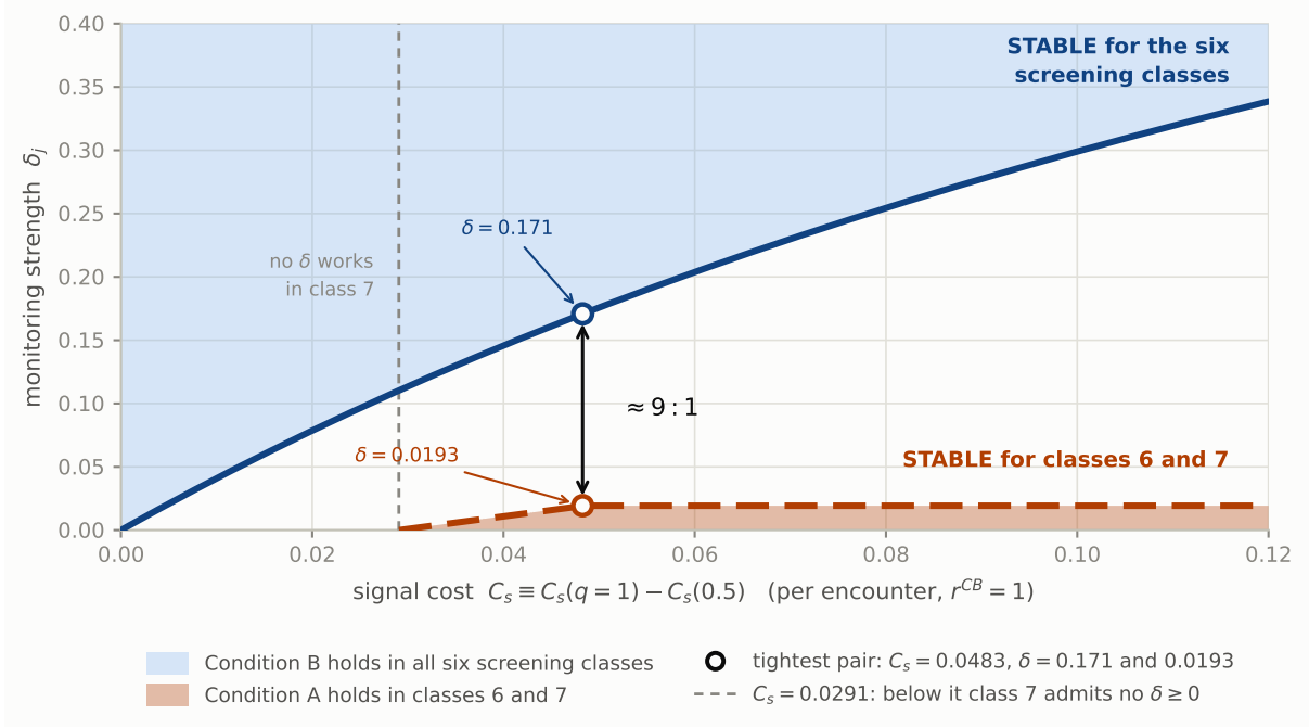
Figure 5: Monitoring strength that sustains the calibrated precision, against the cost of the signal. Horizontal axis: the price of a perfect signal over no signal, C_s \equiv C_s(q=1) - C_s(0.5) , per firm approached, in the units of the calibration ( r^{CB} = 1 ). Vertical axis: the monitoring strength \delta_j of (6), the fraction by which full precision cuts the risk-adjusted cost of lending to each type. The upper band is where Condition B, C_s \leq L_j , holds in all six classes estimated at \hat{q} \approx 1 ; the lower band is where Condition A, G_j \leq C_s , holds in ratings 6 and 7, estimated at \hat{q} = 0.53 , and success probabilities stay below one. Both bands exist for C_s \geq 0.029 , so all eight estimates are stable, but they never overlap: the smallest spread between them, 0.171 against 0.0193 or about nine to one, is reached at C_s = 0.0483 and is marked. Computed at the estimates of Table 4; Appendix F gives the two conditions and the class-by-class bounds.
