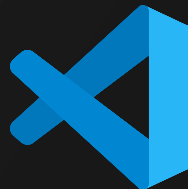
VsCode
