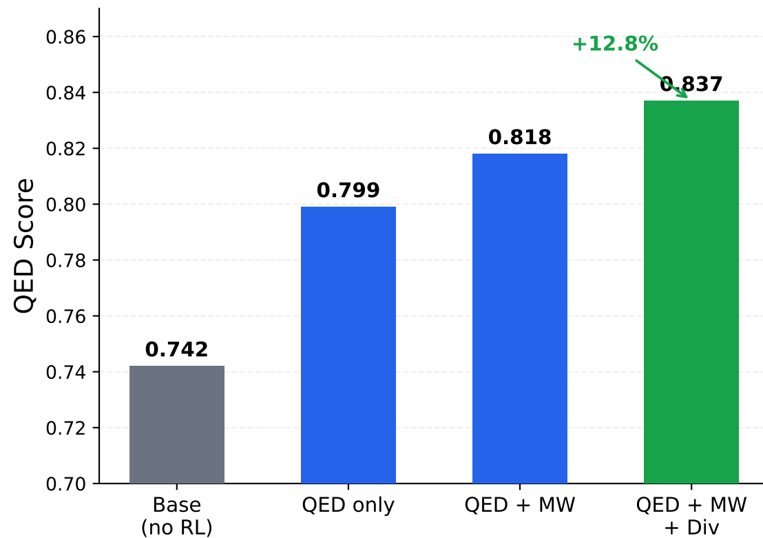
Drug-likeness (QED)
