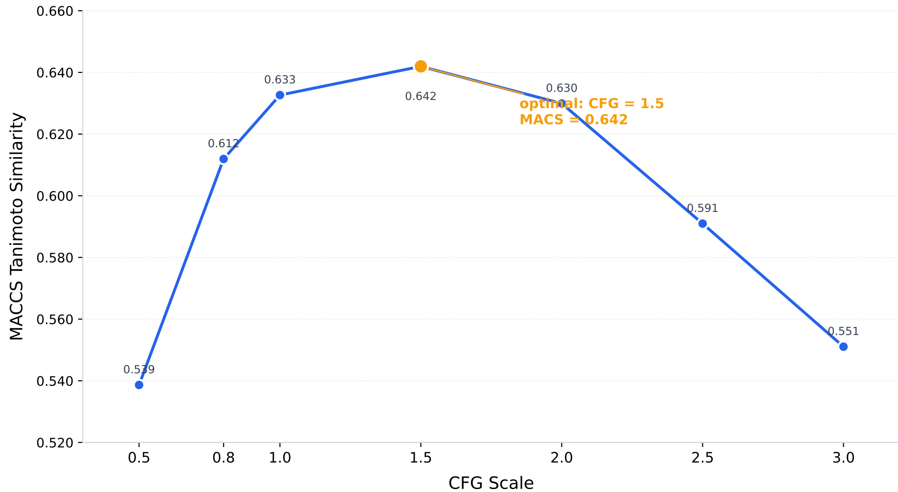
CFG Scale Sweep — SciBERT 20ep on MACCS (temp=0.6, steps=50)
