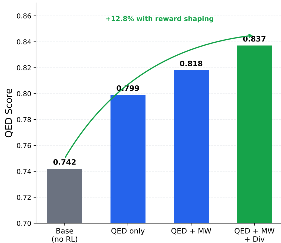
Drug-likeness (QED)
