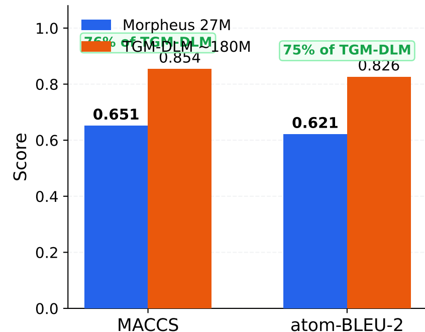
Performance (MACCS & atom-BLEU-2)
