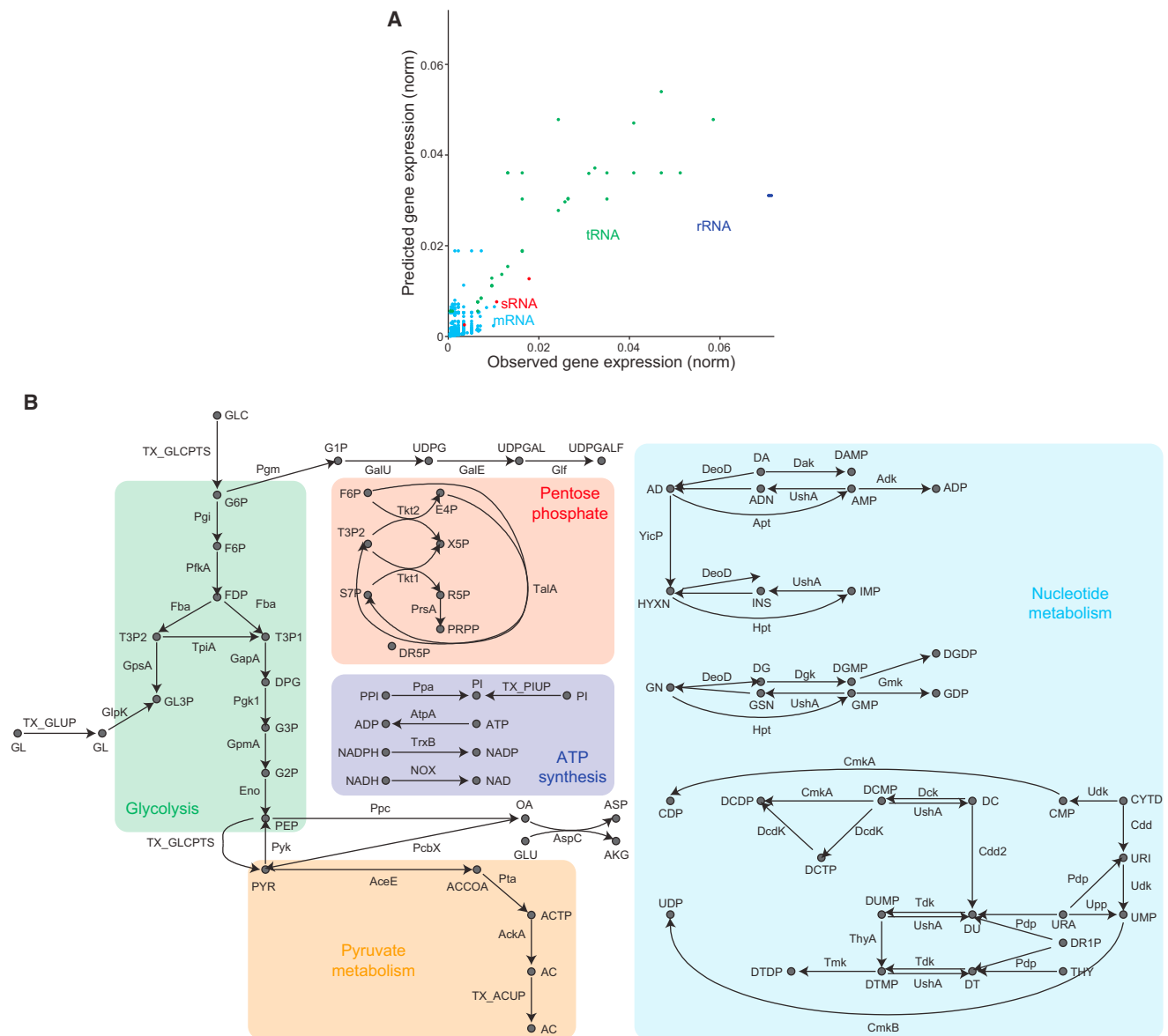
Figure S1. Model Was Trained Using Observed Gene Expression Data, and It Reproduces Metabolic Data, Related to Figure 2
