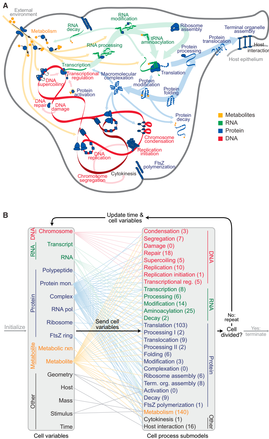
Figure 1. M. genitalium Whole-Cell Model Integrates 28 Submodels of Diverse Cellular Processes
