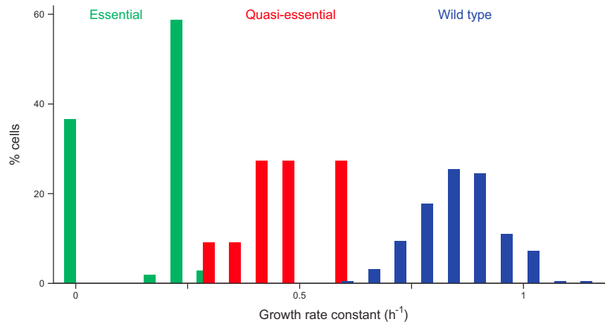
Figure S2. Quasiessential and Essential Single-Gene Disruption Strains Exhibit Significantly Reduced Growth, Related to Figure 6
