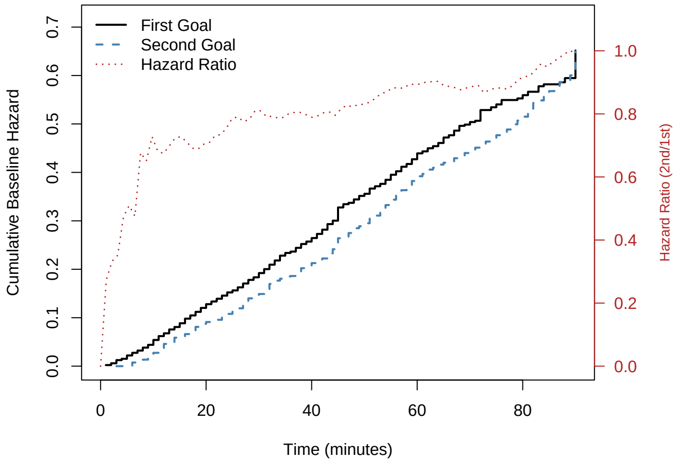
Figure 1: Cumulative Baseline Hazard (Model VII)
