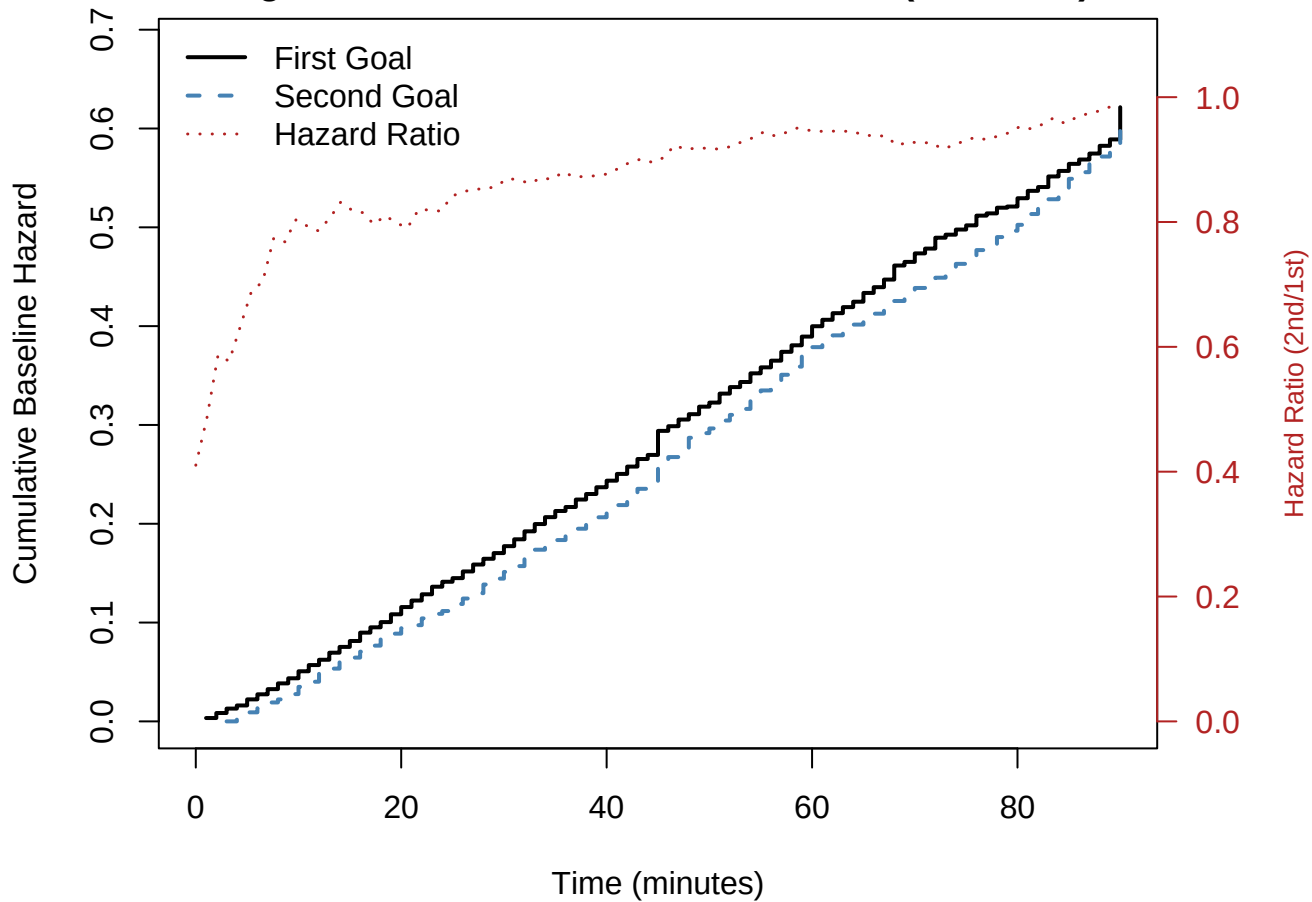
Figure 1: Cumulative Baseline Hazard (Model VII)
