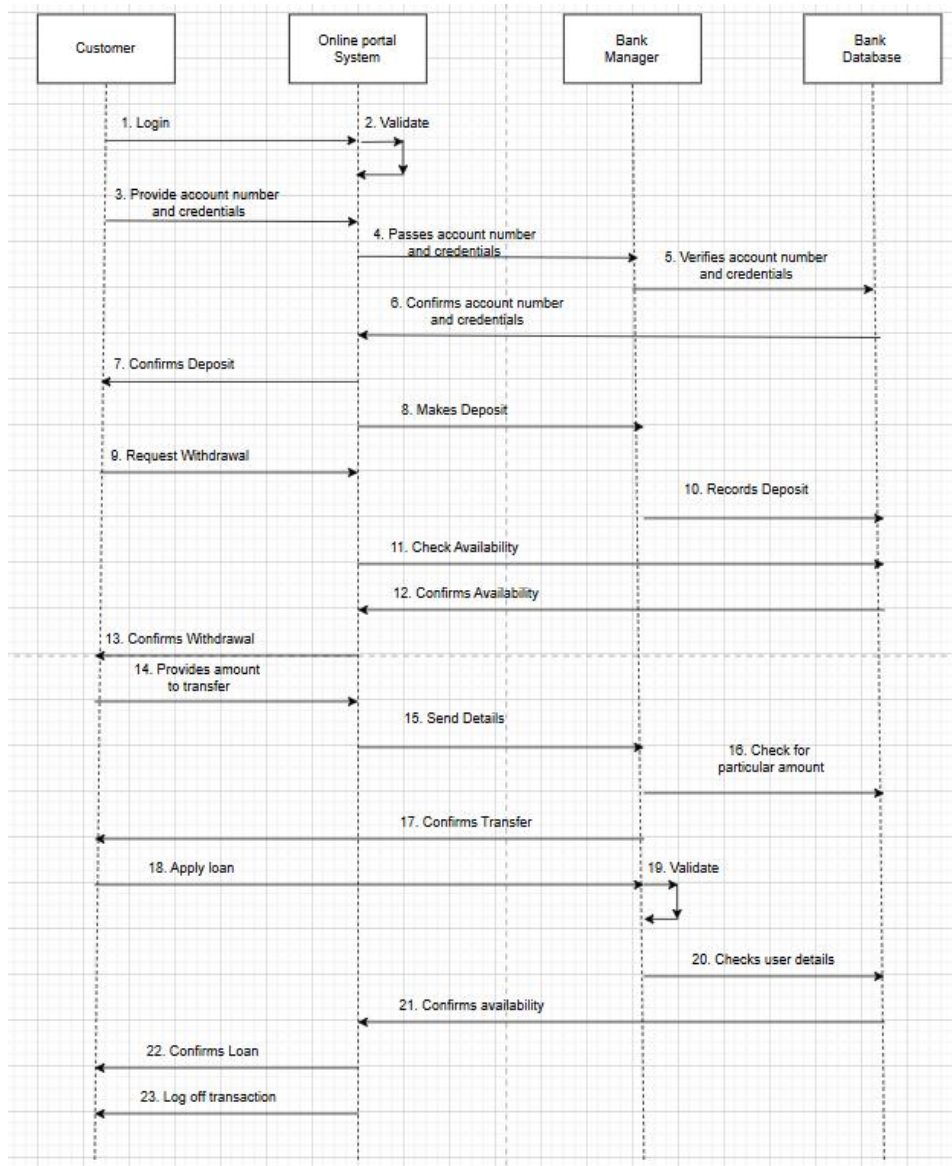
Fig. 4.2 Sequence diagram of Online Banking system
