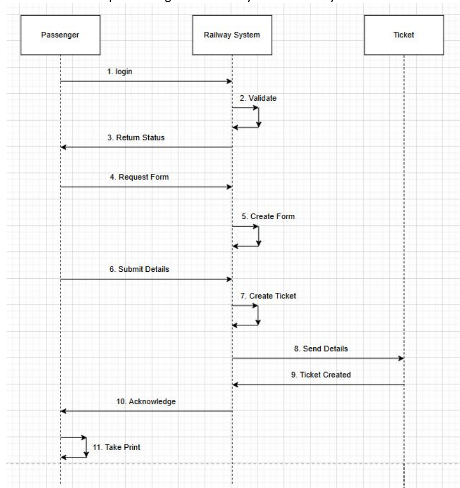
Fig. 4.1 Sequence diagram of Railway Reservation system
