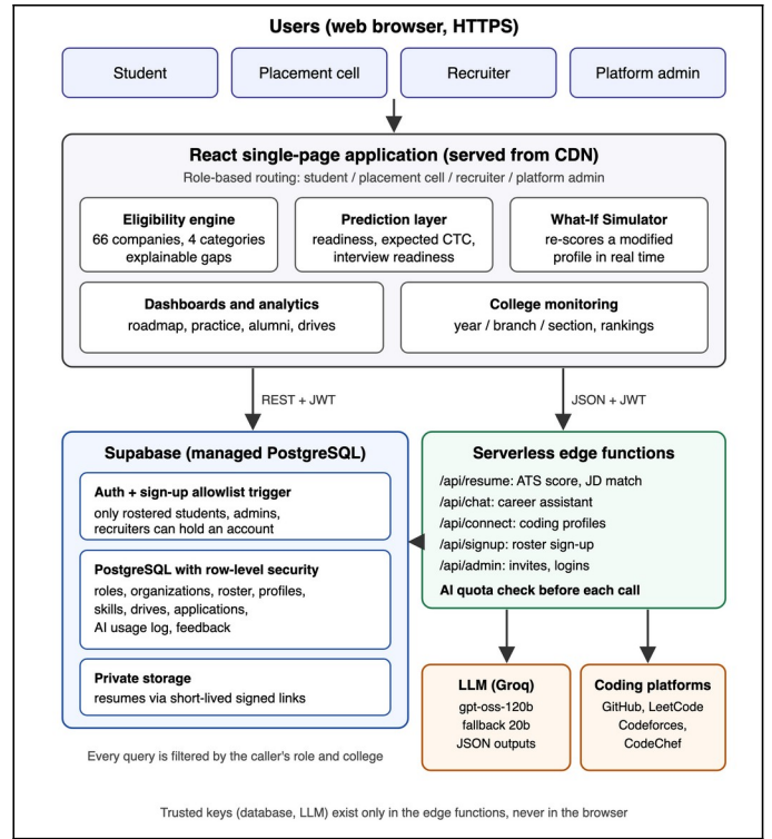
Fig. 1. Proposed system architecture of PlacementIQ Enterprise.
