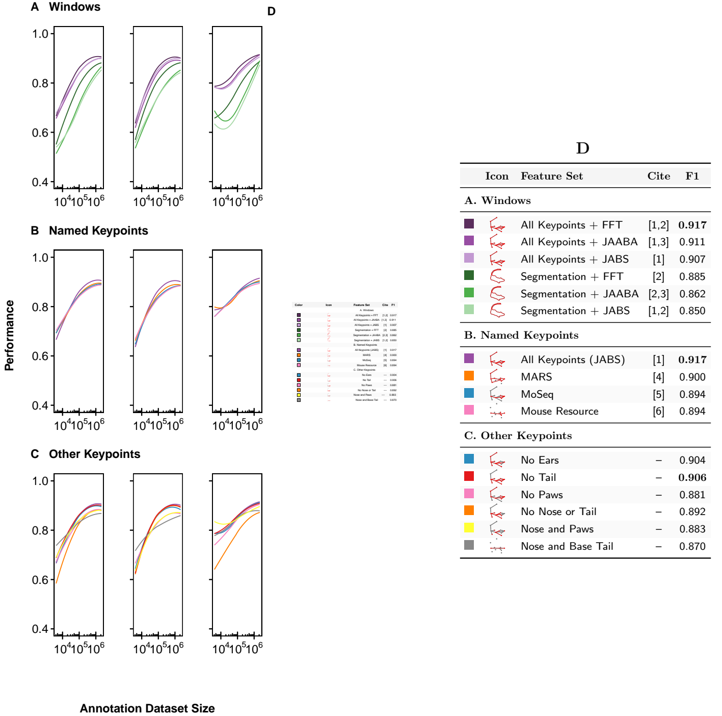
Figure 1: Performance of grooming classification across different feature representations. (A) Comparison of window feature types (FFT, JAABA, JABS) for All Keypoints vs. Segmentation representations. (B) Named keypoint representations from different published sources. (C) Ablation study with keypoint subsets. (D) Legend showing color coding, skeleton icons, and F1 scores for each feature set. Bold indicates best performance per category.
