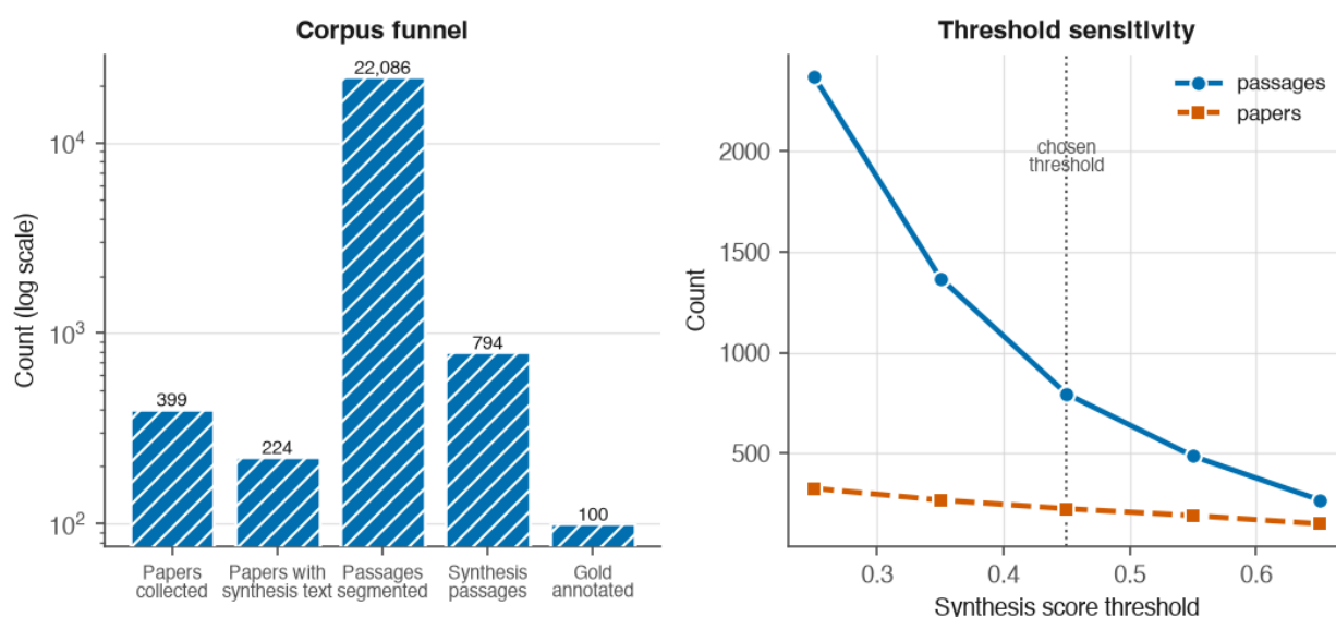
Figure 1. Left, the corpus funnel from collection to the gold standard, on a log scale because each stage is roughly an order of magnitude smaller than the last. Right, the same threshold sensitivity as the table, shown as a curve so the chosen cutoff of 0.45 can be seen sitting on the shoulder of the curve rather than at an arbitrary point on a steep slope.
