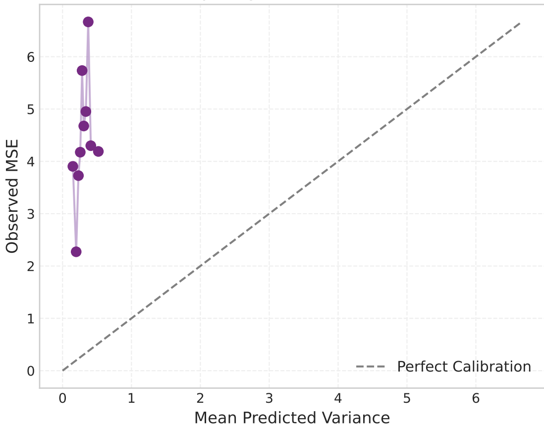
Reliability Diagram (Variance vs Error)
