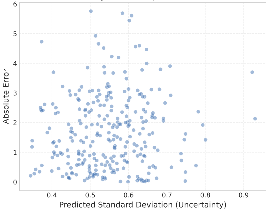
Uncertainty vs Error (Spearman = 0.085)
