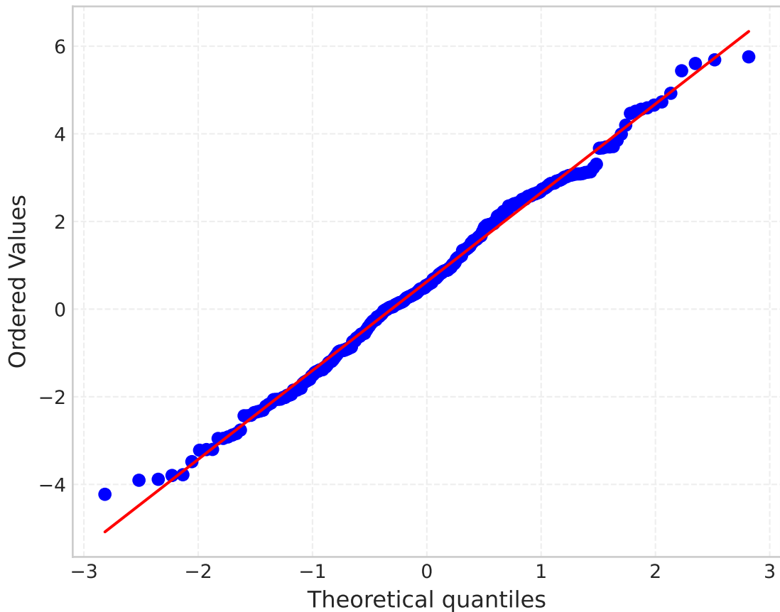
Residual QQ Plot
