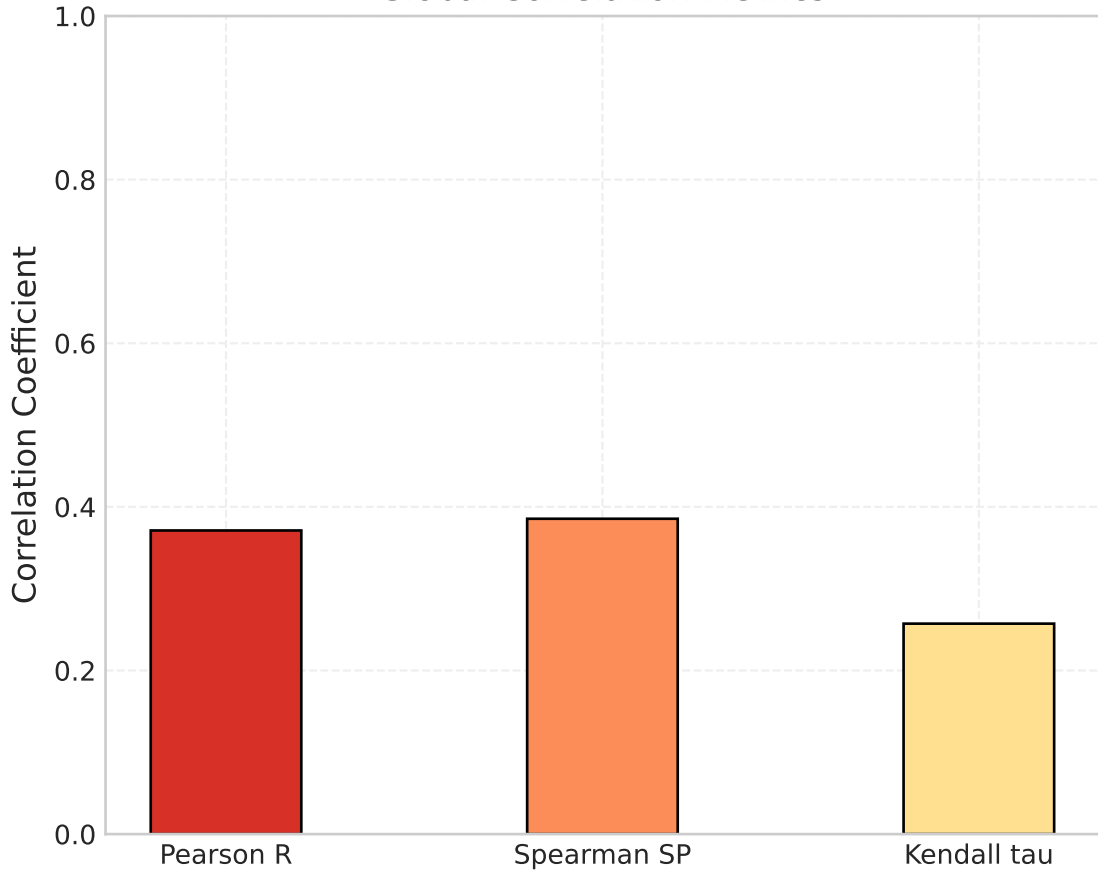
Global Correlation Metrics
