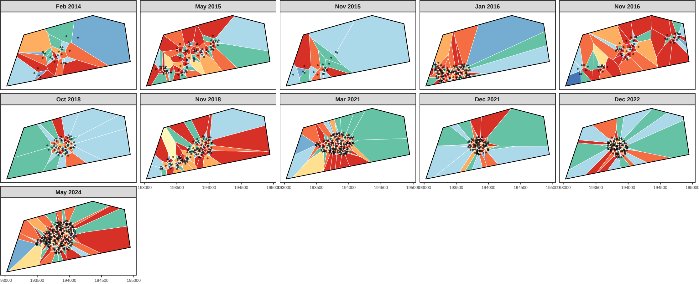
Voronoi tessellation — Velavadar_LEK2 (CSR) coloured by neighbour count
