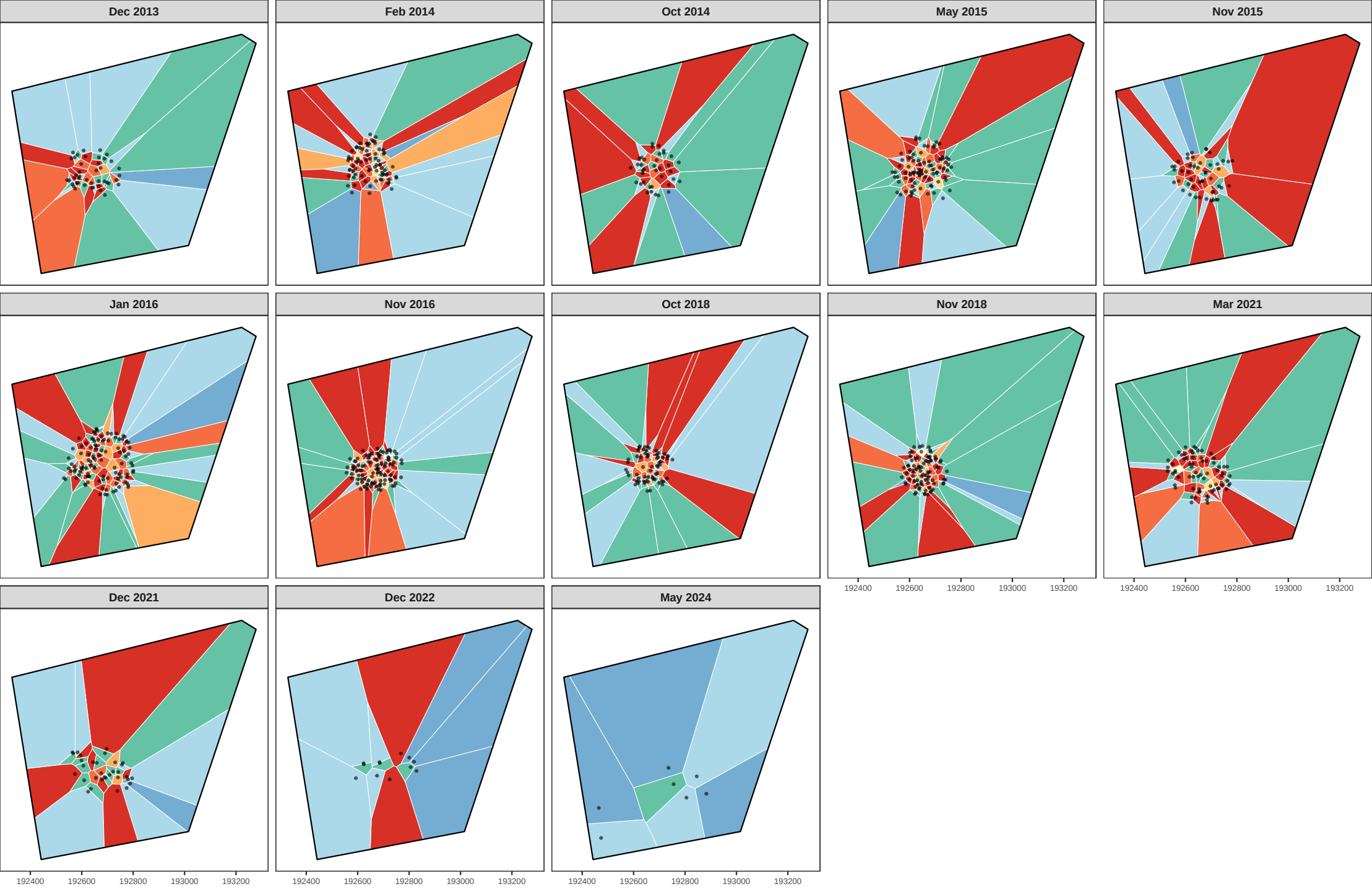
Voronoi tessellation — Velavadar_LEK1 (CSR) coloured by neighbour count
