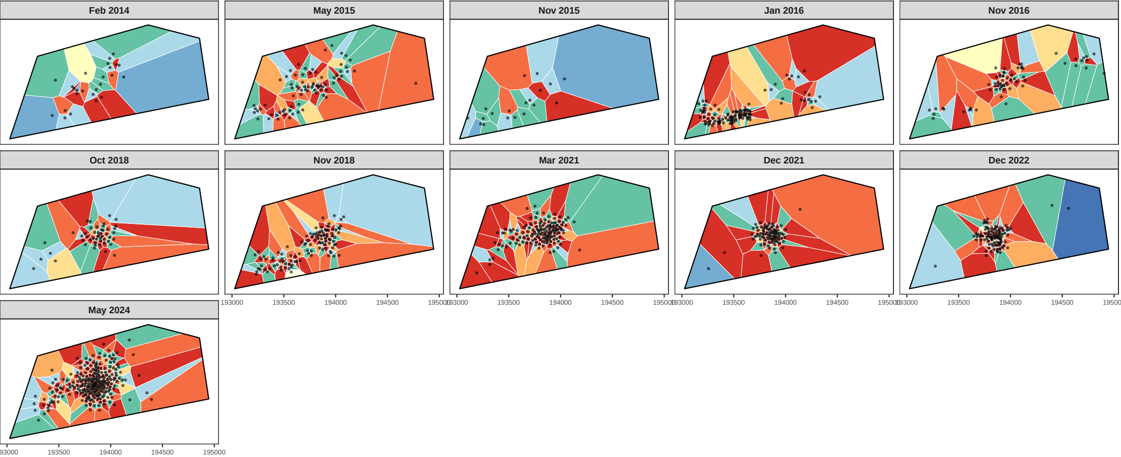
Voronoi tessellation — Velavadar_LEK2 (observed) coloured by neighbour count
