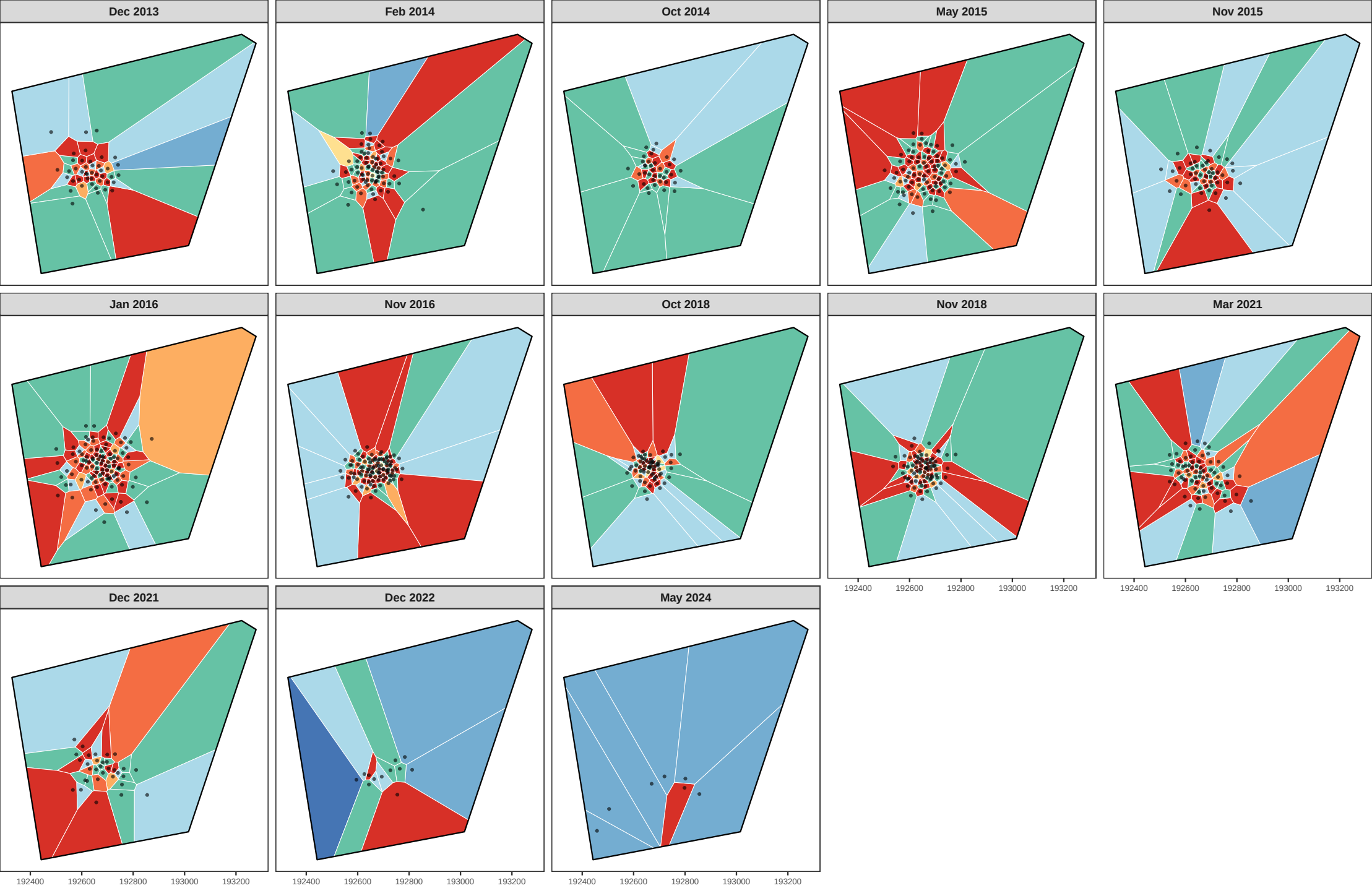
Voronoi tessellation — Velavadar_LEK1 (observed) coloured by neighbour count
