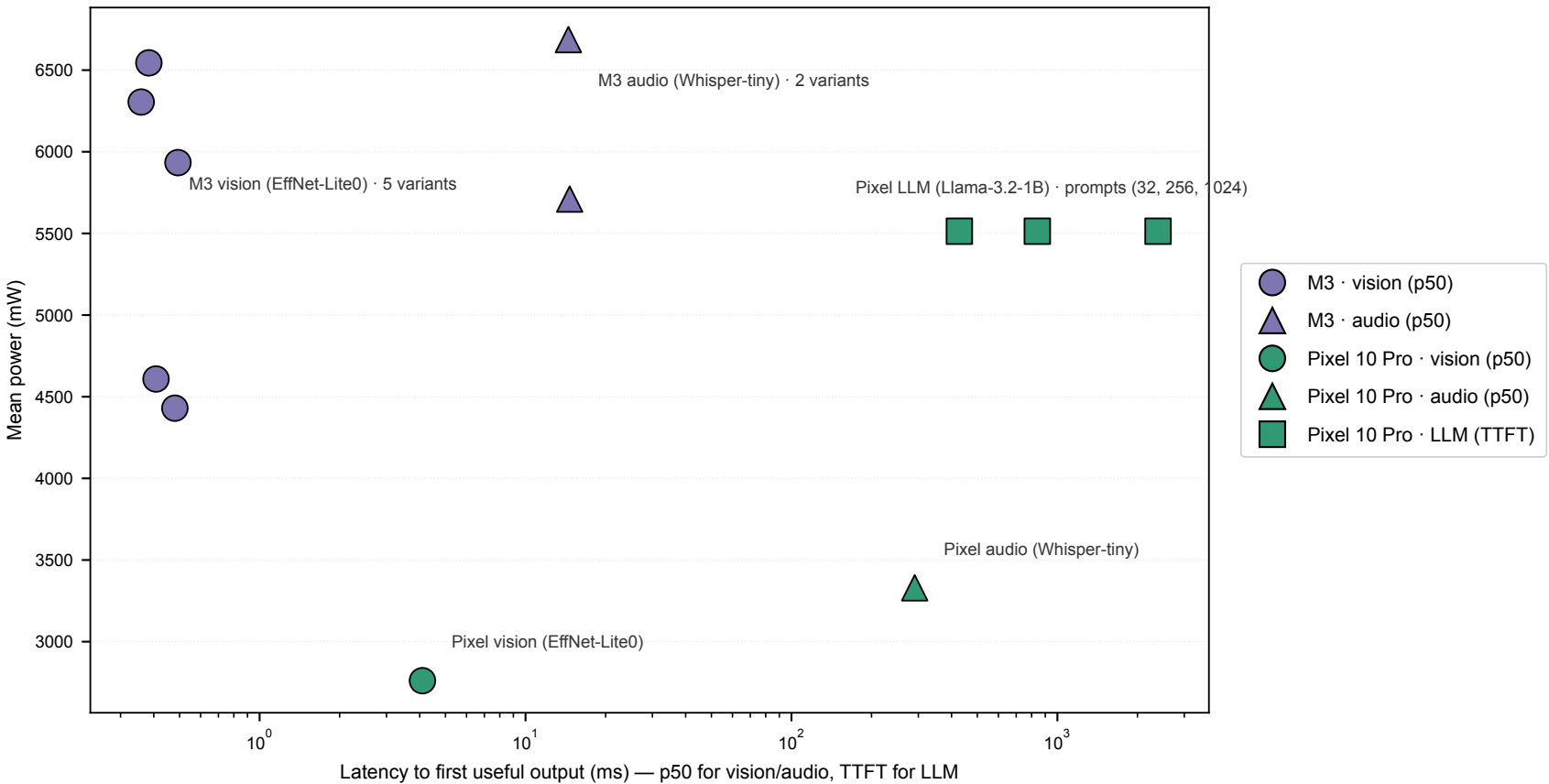
11.1.1 — Cross-modal design space: latency × power on shipped devices
