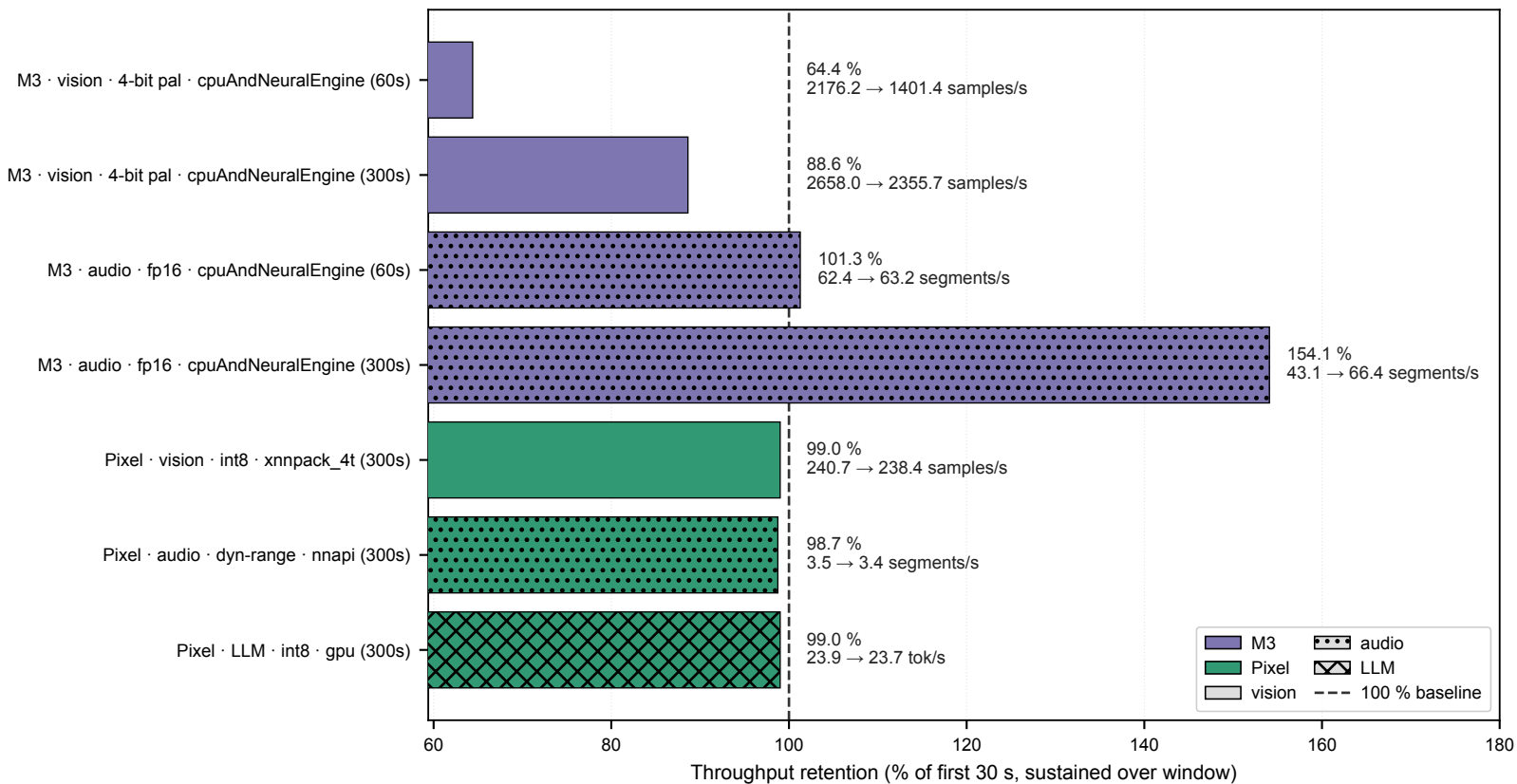
11.1.2 — Thermal retention across modalities × devices (100 % = no throttle; lower bars throttled)
