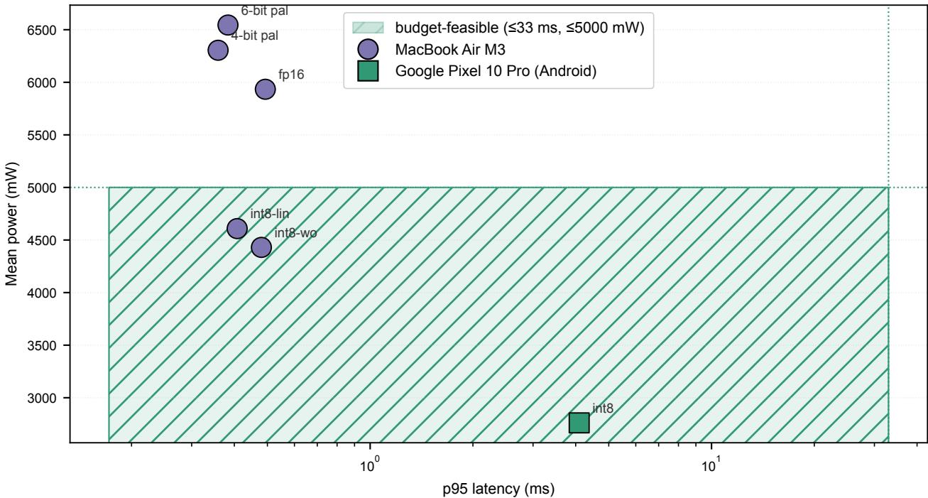
11.1.3 — EfficientNet-Lite0 budget-feasible region ( p_{95} \leq 33 ms, mean power \leq 5000 mW)
