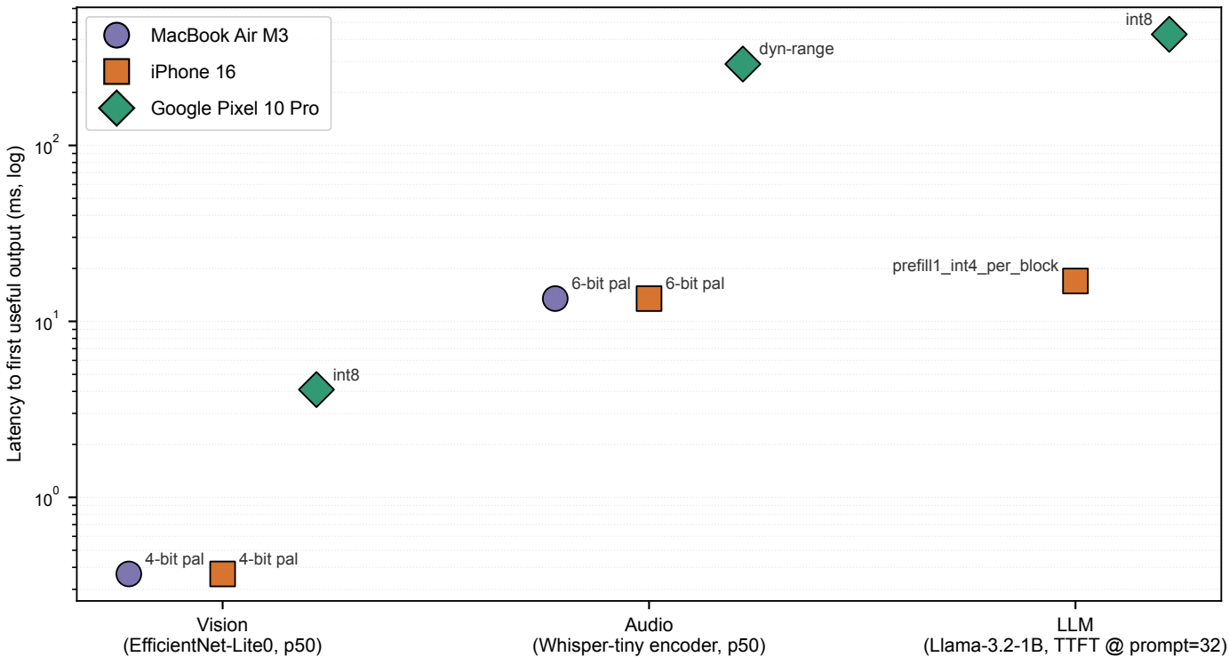
11.1.4 — Cross-modal latency on shipped devices (canonical per-modality config)
